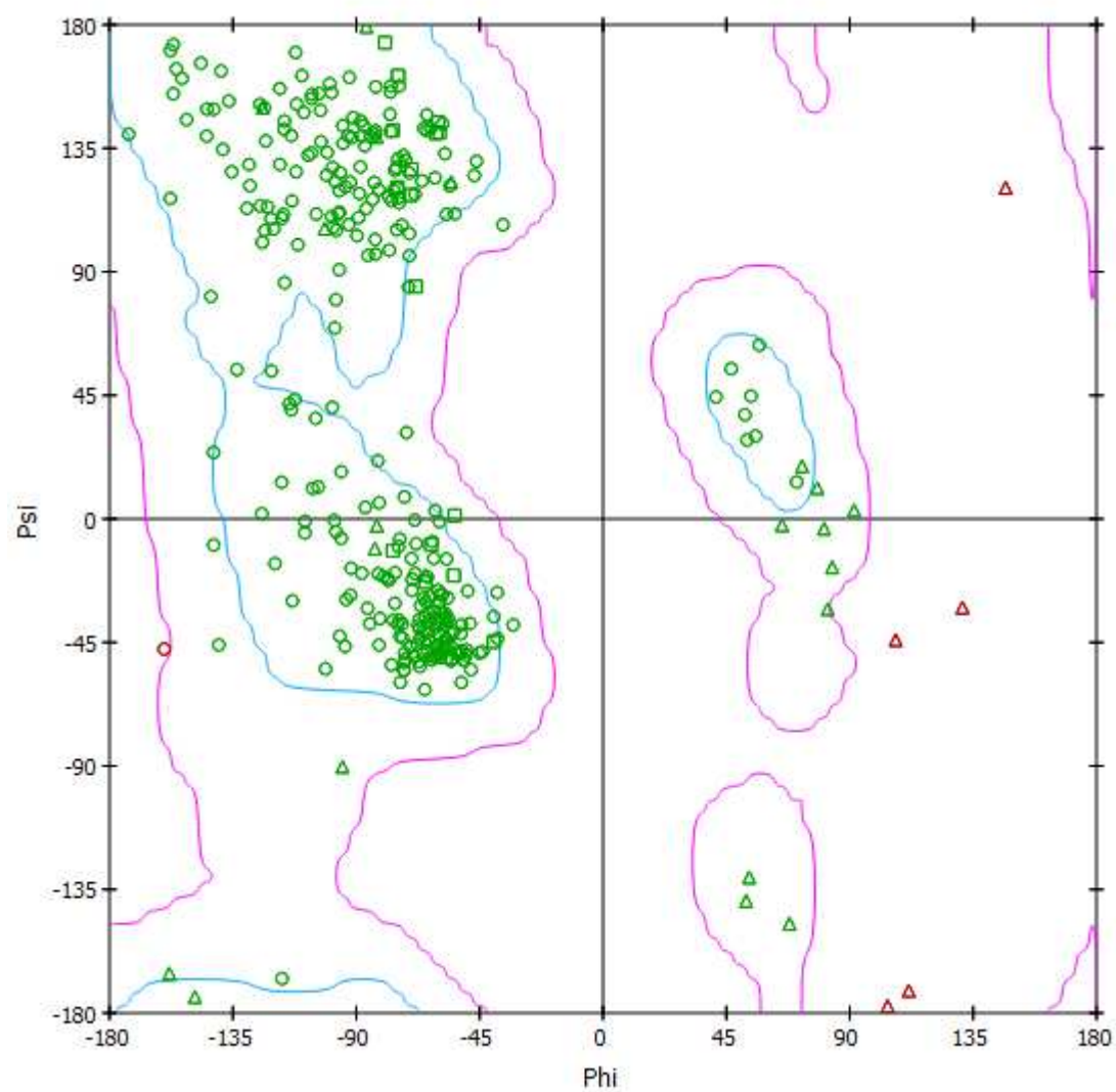
Ramachandran plot
