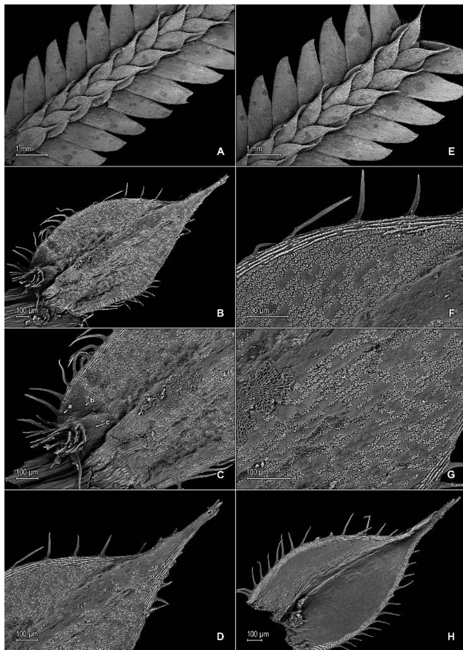
Figure 1. Selaginella nanuzae Valdespino. A Section of upper surface of stem B Upper surface of median leaf C Close-up of base and proximal portion of median leaf, upper surface; note marginal (a) and submarginal (b) stoma, and outer base tufted with long cilia (c) D Close-up of distal portion and apex of median leaf, upper surface E Section of upper surface of stem F Close-up of outer half of median leaf, upper surface G Close-up of inner half of median leaf, upper surface H Lower surface of median leaf. A–H taken from the holotype, Salino et al. 7788 (PMA).
