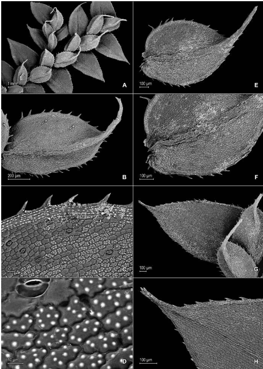
Figure 11. Selaginella trygonoides Valdespino. A Section of upper surface of stem B Upper surface of median leaf; note submarginal stomata (a) on inner half of the lamina C Close-up of inner margin of median leaf, upper surface; note submarginal stomata (a) D Close-up of median leaf upper surface; note papillae on cell lumen E Upper surface of median leaf; note submarginal stomata on inner half of the lamina F Close-up of base, portion of inner margin and inner half of lamina (note stomata), and portion of outer margin and outer half of lamina of median leaf, upper surface G Upper surface of lateral leaf and portion of median leaves, upper surface H Close-up of distal portion and apex of lateral leaf, upper surface. A–H taken from the holotype, Almeida et al. 1994 (PMA).
