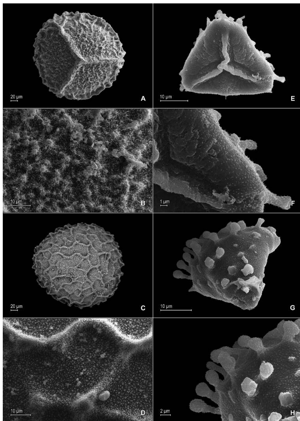
Figure 9. Selaginella pellucidopunctata Valdespino. A Megaspore, proximal face B Close-up of megaspore, proximal face C Megaspore, distal face D Close-up of megaspore, distal face E Microspore, proximal face F Close-up of microspore, proximal face G Microspore, distal face H Close-up of microspore, distal face. A–H taken from the isotype, Oliveira 1094 (PMA).
