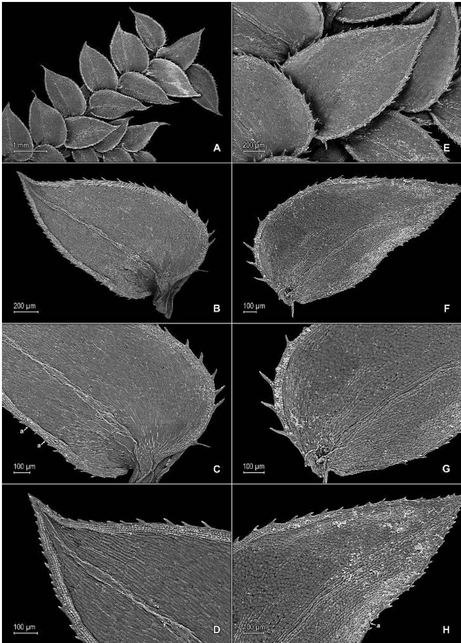
Figure 12. Selaginella trygonoides Valdespino. A Section of lower surface of stem B Lower surface of lateral leaf C Close-up of base and proximal portion of lateral leaf, lower surface; note marginal stomata (a) D Close-up of distal portion and apex of lateral leaf, lower surface E Lower surface of axillary leaf and portions of lateral leaves F Upper surface of lateral leaf G Close-up of base and proximal portion of lateral leaf, upper surface H Close-up of distal portion and apex of lateral leaf, upper surface; note marginal stoma (a). A–H taken from the holotype, Almeida et al. 1994 (PMA).
