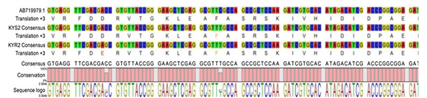
Figure 3. Gene sequencing for the ALS enzyme of the two Kyllinga brevifolia biotypes.
