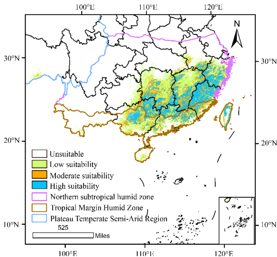
FIGURE 5 Suitable area for D. shixingense under current climate.
