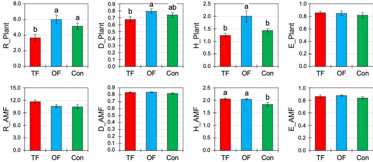
Figure 3. Herb and fungal community diversity (mean \pm SE) under different fire treatments: two fires (TF), one fire (OF), and no fire occurred or control site (Con). R : Menhinick richness; D : Gini-Simpson index; H' : Shannon index; E : Pielou's evenness index. Letter indicates significant differences at p < 0.05 inferred from ANOVA followed by Duncan's multiple range tests.
