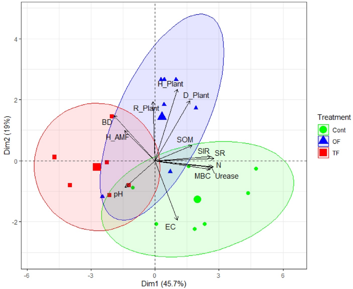
Figure 4. The fire treatment predicts the soil functionalities and the biodiversity. Biplot of principal component analysis (PCA) based on soil physical, chemical, and biological properties, and fungal and plant community diversity indices, under different fire treatments: two fires (TF), one fire (OF), and control site (Con). BD: bulk density; EC: electrical conductivity; pH: soil acidity; SOM: organic matter; N: total nitrogen; SR: soil respiration; SIR: substrate-induced respiration; MBC: microbial biomass carbon; Urease: urease activity; Biodiversity indices: richness (R), Gini-Simpson (D), Shannon (H) for herbs (Plant) of fungi (AMF). Centroid of plots under TF, OF, or Con treatment is indicated by a greater shape (red square: TF; blue triangular: OF; green circle Con). Ellipses denote the perimeter of plots per treatment.
