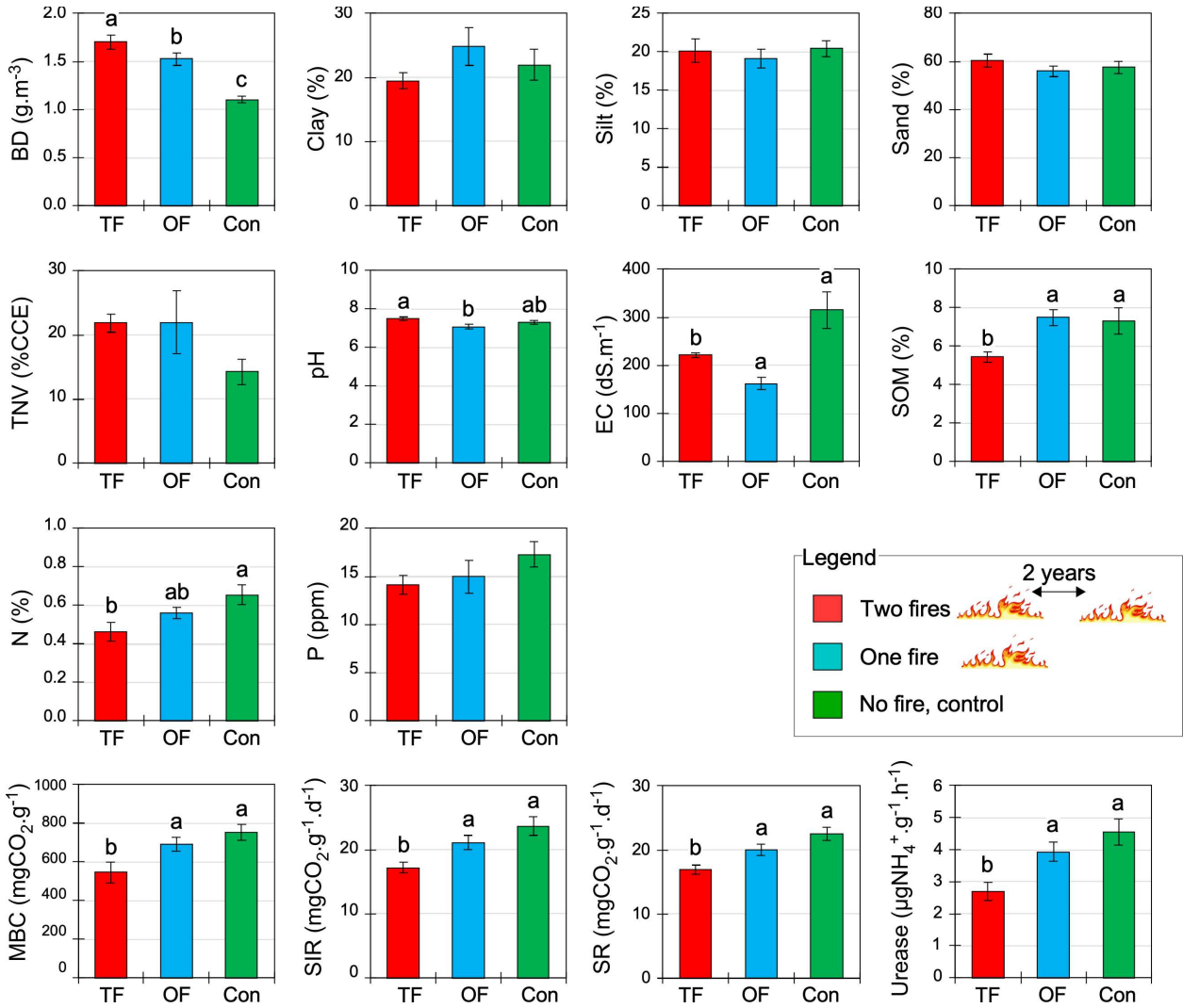
Figure 2. Soil physical, chemical, and biological properties (mean \pm SE) under different fire treatments: two fires (TF), one fire (OF), and no fire occurred or control site (Con). BD: bulk density; TNV: total neutralizing value; EC: electrical conductivity; SOM: soil organic matter; pH: soil acidity; N: nitrogen; P: phosphorus; MBC: microbial biomass carbon; SR: soil respiration; SIR: substrate-induced respiration; Urease: soil urease enzymatic activity. Letter indicates significant differences at p < 0.05 inferred from ANOVA followed by Duncan's multiple range tests.
