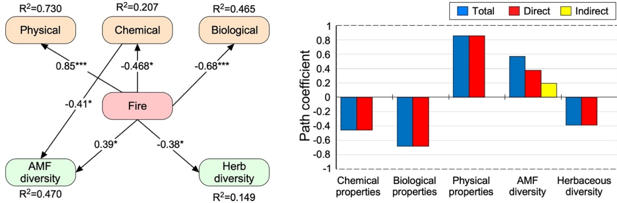
Figure 5. Direct and indirect effects of fire treatment. The best fit structural equation modeling (SEM) on the best variables in different groups of soil physical, chemical, and biological and plant and fungal species diversity indices. The values adjacent to lines are standardized path coefficients. * and *** indicate the significant paths at 0.05 and 0.001, respectively.
