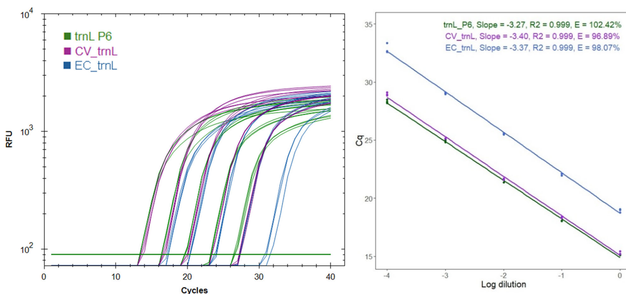
Fig. 1 | Primer efficiencies. Amplification of trnL P6 —, CV_ trnL —, and EC_ trnL — markers with a standard curve of honey extract (1X – 10,000X diluted). The raw data (RFU) and regression ( C_q ) are marked. The three technical replicates are shown for each reaction.
