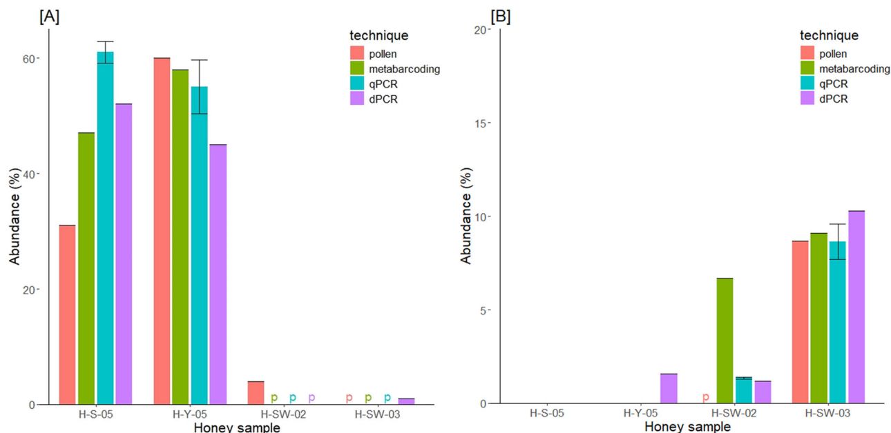
Fig. 2 | Results from melissopalynology, metabarcoding, qPCR and dPCR for detection of C. vulgaris and Erica spp. Comparison of methods used to quantify [A] Calluna vulgaris and [B] Erica spp. in four UK heather honey samples where “p” indicates a presence at < 1%. The methods used were: pollen (melissopalynology)
