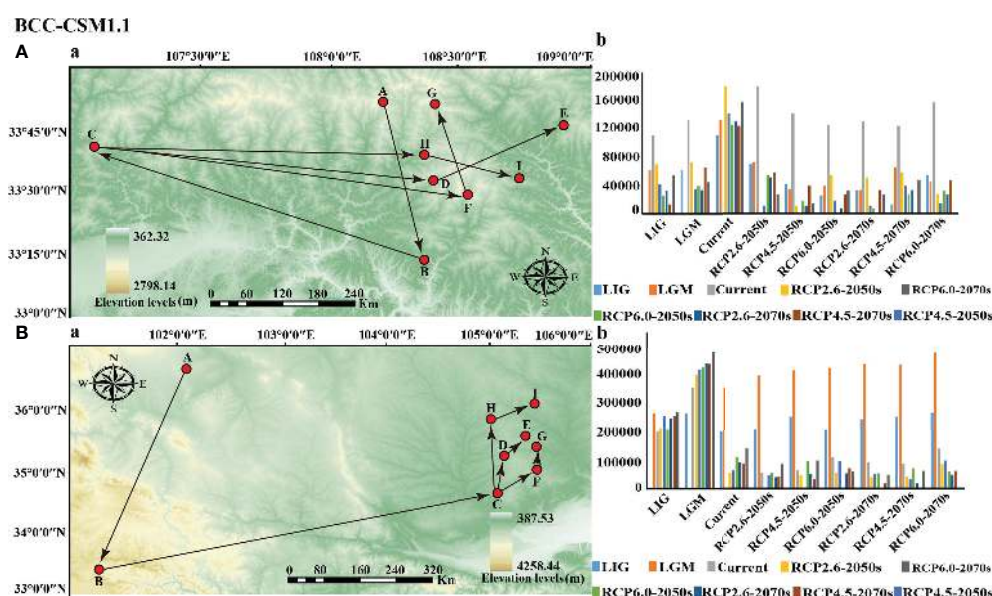
FIGURE 8 Migration of the center of suitable habitat for two subspecies of P. rockii since the last interglacial period (A: P. rockii subsp. rockii ; B: P. rockii subsp. taibaishanica ; (a) migration route; (b) migration distance). Among them, the meaning of the letters were (A) LIG, (B) LGM, (C) current, (D) RCP2.6-2050s, (E) RCP2.6-2070s, (F) RCP4.5-2050s, (G) RCP4.5-2070s, (H) RCP6.0-2050s, (I) RCP6.0-2070s.
