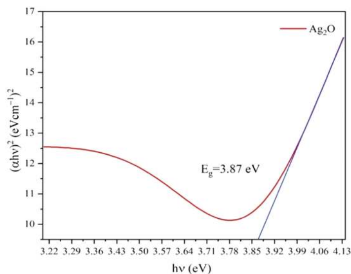
Figure 3 Tauc's plots for the band gap energy of \text{Ag}_2\text{O} NPs.
