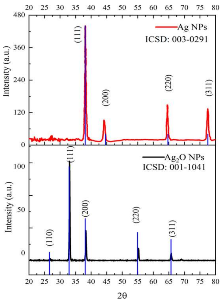
Figure 4 XRD patterns of Ag and \text{Ag}_2\text{O} NPs.
