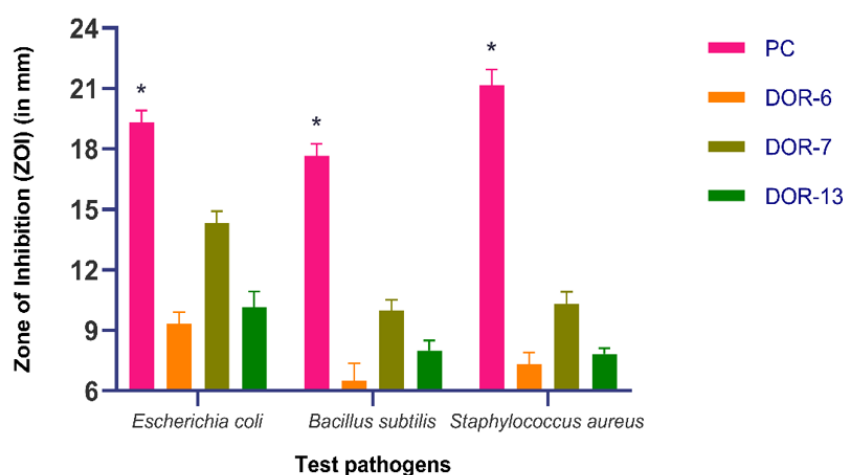
Figure 15. Comparison of antimicrobial activity of fungal extracts DOR-6, DOR-7 and DOR-13 with positive control. Comparison of mean zones of inhibition measurements (mm) of fungal crude extracts (DOR-6, DOR-7 and DOR-13) with antibiotic - 10 \mu g Gentamycin disc, as a positive control (PC) for bacterial test pathogens. Error bars represent standard deviation. An asterisk indicates significant difference in mean zones of inhibition between positive control and fungal crude extracts observed for each test pathogen (compared using Dunnett's test, P < 0.05 ). The less potency of the fungal extract in comparison to antibiotic disc of Gentamycin can be attributed to the crude nature of the extracts used. If no inhibition was seen, a value of 6 was assigned, which was the diameter of the agar-well used.
