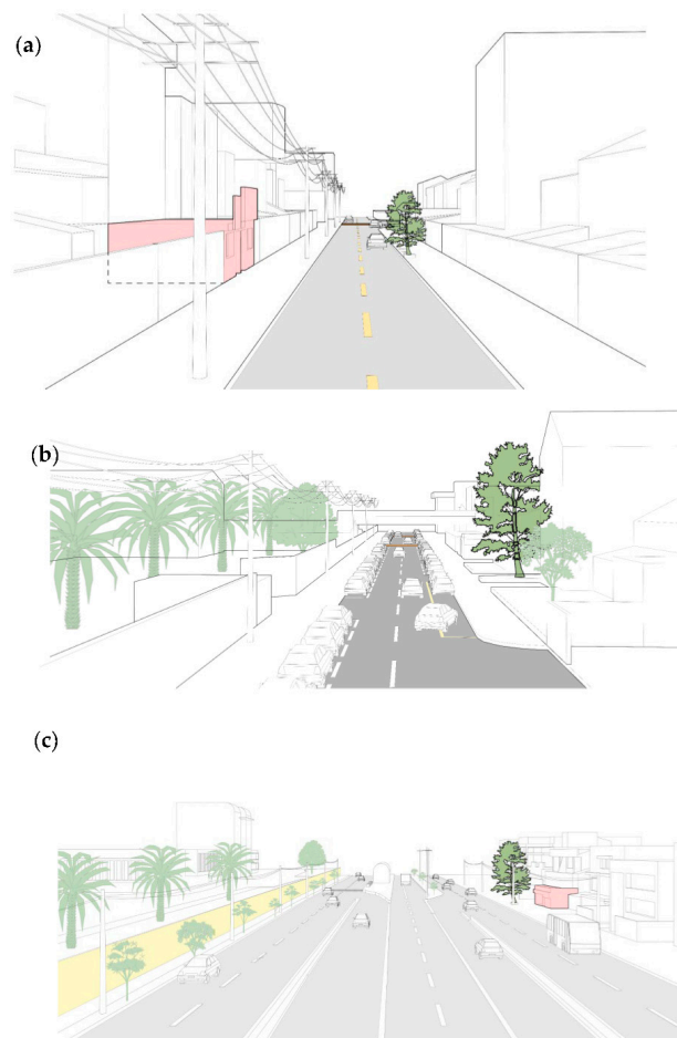
Figure 2. Visual description of: (a) a shallow canyon street (Point S19); (b) a wide road (Point S7); (c) and open road (Point S14), with mobile (cars) and stationary sources (restaurants, in red), and sampled trees bordered in black.
