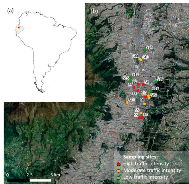
Figure 1. Study area: (a) Location of Quito (colored point), Ecuador (gray fill), on the map of South America; (b) study sites in Quito.
