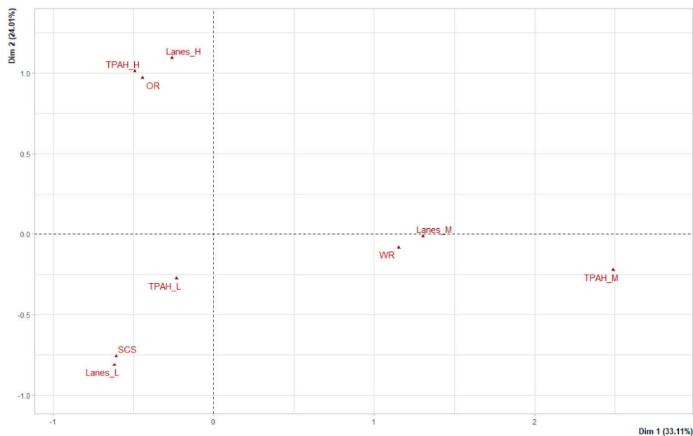
Figure 6. Representation of the variables of the multiple correspondence analysis. TPAH_H, higher total concentrations of PAH; Lanes_H, higher number of lanes; OR, open roads; TPAH_L, lower total concentrations of PAHs; SCS, shallow canyon streets; Lanes_L, lower number of lanes; Lanes_M, medium number of lanes; WR, wide road; TPAH_M, medium total concentrations of PAHs.
