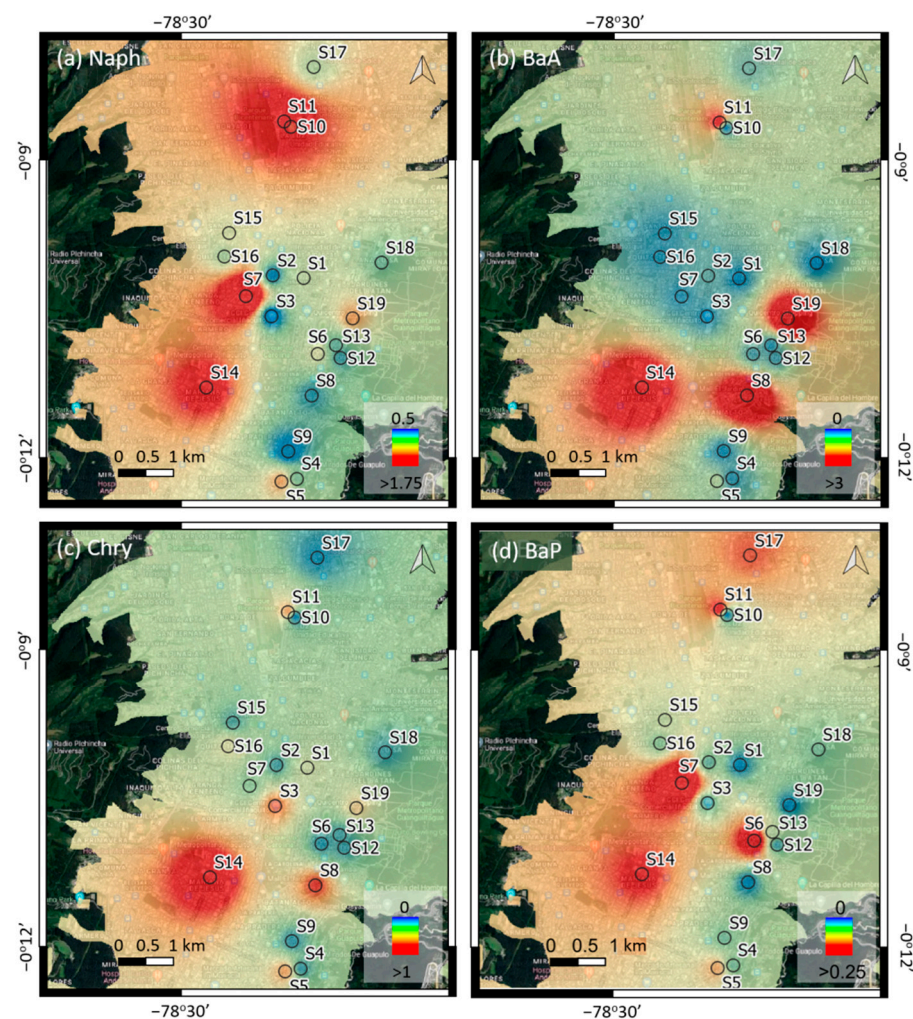
Figure 4. Distribution patterns of the concentration of PAHs studied in the city of Quito.
