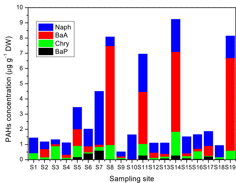
Figure 3. Total and individual concentration of PAHs in needle samples at all sites studied.
