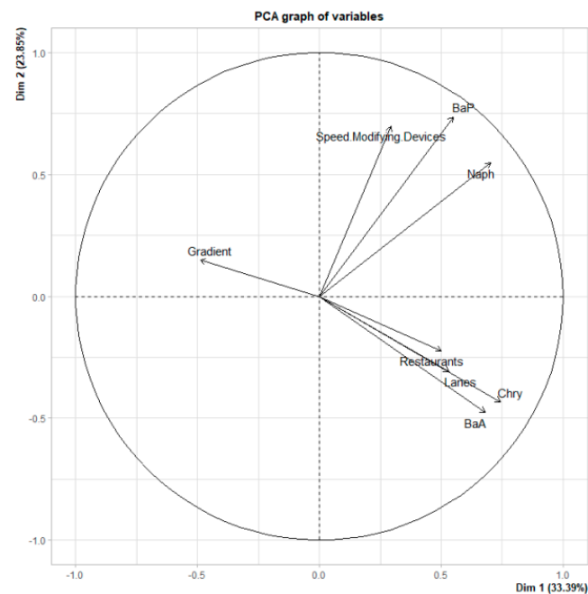
Figure 5. Graph of the variables of the principal component analysis. Naph, naphthalene; BaA, benzo[ a ]anthracene; Chry, chrysene; BaP, benzo[ a ]pyrene.
