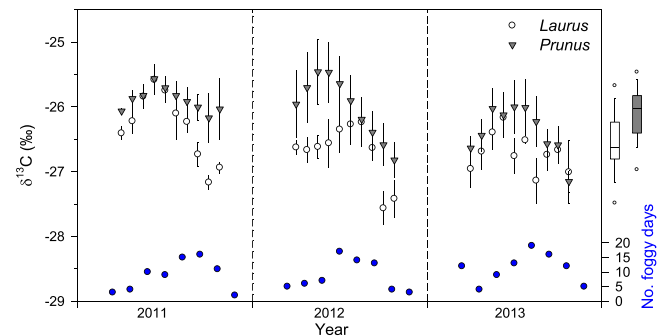
Fig. 3. Intra-annual wood \delta^{13}\text{C} values for the period 2011–2013 for Laurus novocanariensis (white circles and boxplot) and Prunus lusitanica (grey triangles and boxplot). Values are means \pm SE and 2012 was the drought year. The blue circles show the 10-day number of foggy days from March to October. Boxplots show the distribution of \delta^{13}\text{C} values for the two species.
