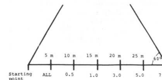
Fig. 1. Plan view of a sample line making up one side of a fuel loading triangle. The amount and composition of slash is measured along each side of the triangle. In the first five meters all intersections with slash are counted, in the next five meters the minimum diameter of slash counted is 0.5 cm and so on until the end of the sides.
