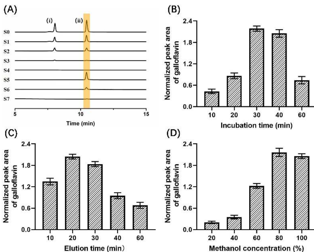
Fig. 8. Effects on the binding efficiency of galloflavin. (A) Base peak chromatograms acquired from different solutions (S0–S7) during the developed LDH-MNPs-based ligand fishing procedure from a model mixture containing chlorogenic acid (i), galloflavin (ii). (B) Incubation times. (C) Elution time. (D) Methanol concentration.
