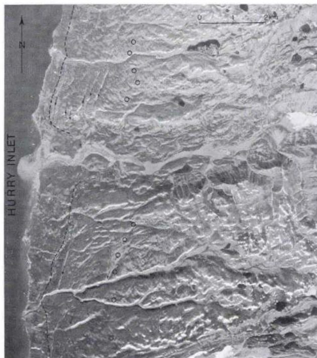
Fig. 10. The east side of Hurry Inlet. Line of open circles denote upper limit of 'fresh' till cover (c. 300 m above sea level). Broken line marks the upper limit of marine and marine-deltaic deposits. Arrows mark lateral drainage channels and kame terraces (The Milne Land Moraines). Copyright Geodetic Institute.
