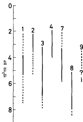
Fig. 23. Dating of the 'climatic optimum' from pollen analytical evidence in different parts of Greenland. Numbers refer to the locality numbers in fig. 22 which also states individual authors.
