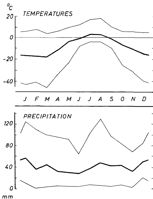
Fig. 2. Temperatures and precipitation at Kap Tobin (Scoresbysund) in the period 1964–1973. Thick lines: average values; thin lines: absolute maximum and minimum values. From Publikationer fra det danske Meteorologiske Institut .
