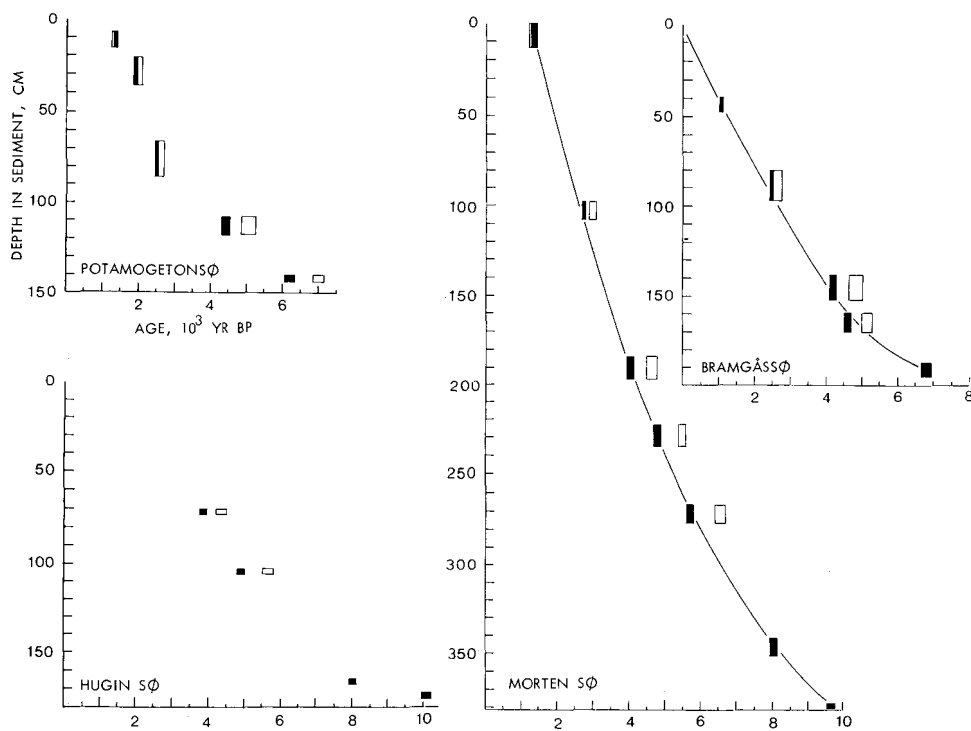
Fig. 13. Age/depth relation of lake sediments. Horizontal length of rectangles represents \pm 1 standard deviation on C-14 counts, the height marks the dated core interval. Open boxes denote dates corrected according to tree ring chronology after Damon et al. (1972).
