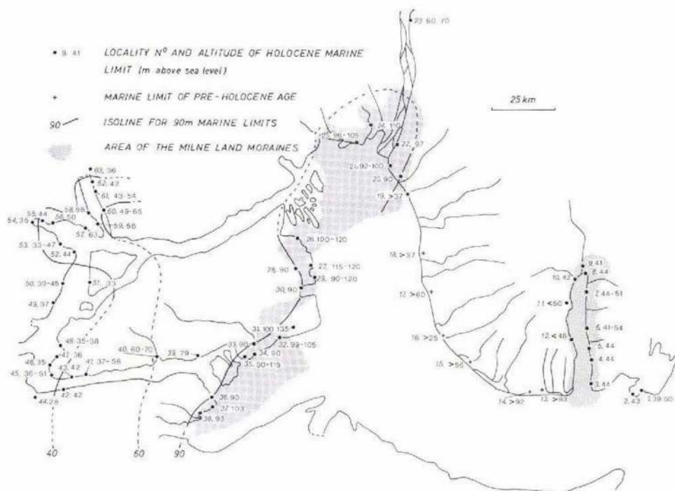
Fig. 4. Marine limits and area of the Milne Land Moraines in the Scoresby Sund region. Locality numbers refer to the list in table 2.
