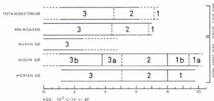
Fig. 15. Dating of pollen interval zones in the Scoresby Sund area.
