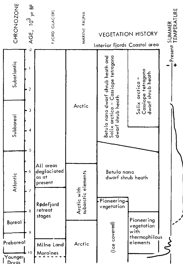
Fig. 24. Correlation of different types of stratigraphical evidence from the Scoresby Sund area, and derived relative summer temperatures.
