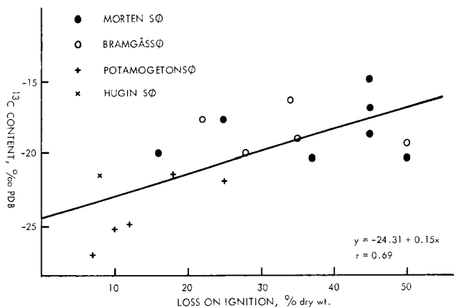
Fig. 12. Regression line for observations on loss on ignition and ^{13}\text{C} content of lake sediments. The correlation coefficient is highly significant ( 1\% > P > 0.1\% ).
