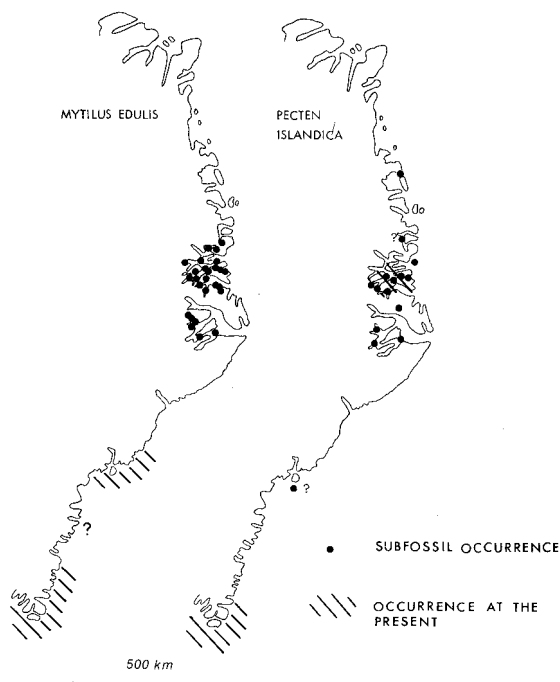
Fig. 6. Past and present distribution of Mytilus edulis and Pecten islandica in East Greenland. Including observations by Hartz ( in Bay, 1895), Nathorst (1901), Jensen (1905, 1917), Noe-Nygaard (1932), Ockelmann (1958), Washburn & Stuiver (1962), Lasca (1969) and Street (1977). Modified from Hjort & Funder (1974).
