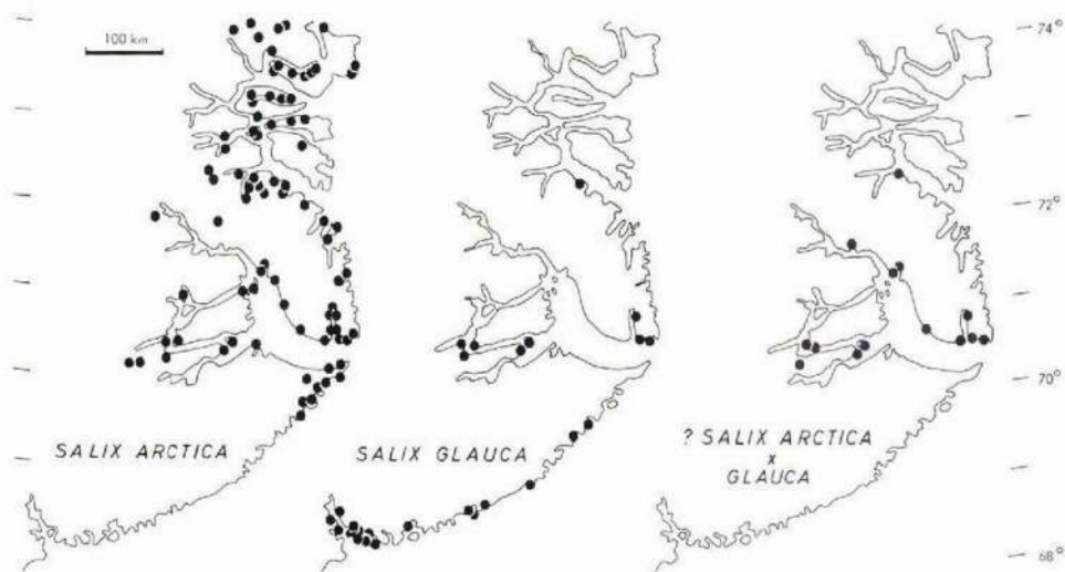
Fig. 20. Distribution of Salix arctica , Salix glauca and their putative hybrids in central East Greenland, according to herbarium specimens at the Botanical Museum in Copenhagen determined by A. Skvortsov.
