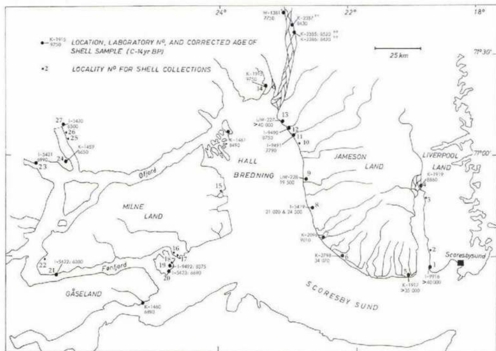
Fig. 3. Shell dates and sites for collection of shell faunas in the Scoresby Sund area. Locality numbers refer to the fauna list, table 3.* from Schafer (in Levin et al. , 1965).** from Street (1977).
