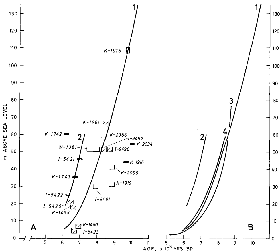
Fig. 5. Emergence curves from the East Greenland fjord zone. A: curves from the Scoresby Sund area, 1: central area (marine limits \geq 90 m), 2: interior fjord area (marine limits \leq 60 m). C-14 dates plotted with \pm one standard deviation. Only hatched samples have been considered in the construction of the curves. Boxes with open tops mark that only minimum values can be determined for corresponding sea level. Black rectangles denote dates on lake sediment, all other dates are on bivalve shells. B: comparison with earlier curves from the fjord zone, 1: central Scoresby Sund, 2: interior Scoresby Sund, 3: Mesters Vig (Washburn & Stuiver, 1962), 4: Skeldal (Lasca, 1969, corrected by the present author according to the principles outlined in the text).
