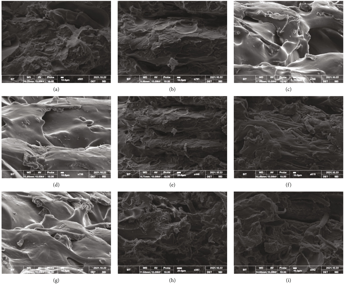
FIGURE 5: Micrographs of tensile fracturegraphy according to Table 2.
