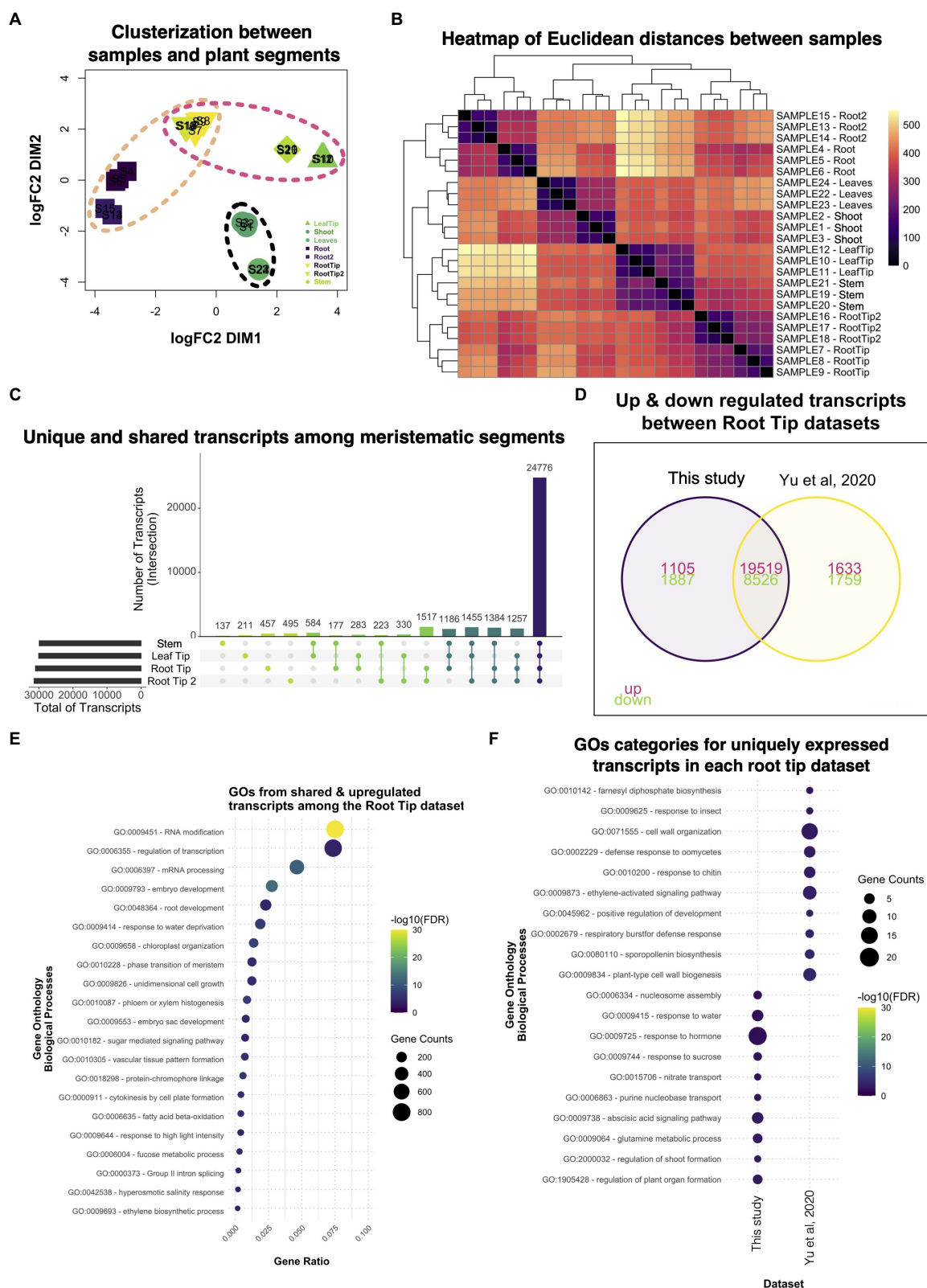
FIGURE 7 Comparative analysis between two different datasets of Ceratopteris sporophytic tissues. (A) Multidimensional scaling analysis to examine how similar and contrasting are the samples and plant parts of both datasets. (B) Heatmap showing the relatedness between samples and plant segments in the two datasets. (C) Plot showing the unique and shared transcripts between meristematic segments. (D) Venn diagram exhibiting how many transcripts are shared or unique among root tip datasets. (E) GO enrichment analysis of the shared transcripts between both root tips samples. (F) GO enrichment analysis of transcripts that are expressed uniquely in each root tip dataset.
