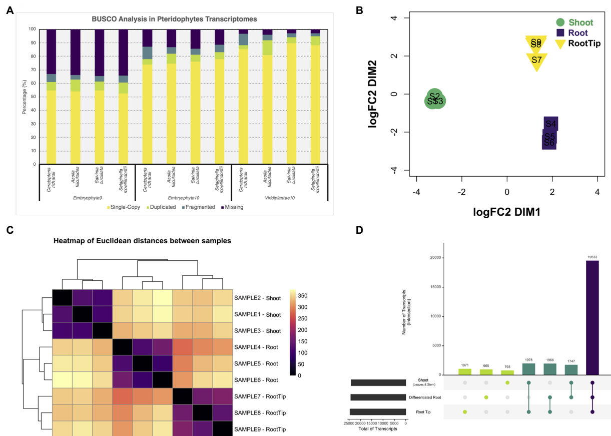
FIGURE 1 Differential gene expression analysis from tissues of Ceratopteris richardii young sporophyte. (A) Comparison of the gene content between pteridophytes transcriptomes using different BUSCO databases. (B) Multidimensional scaling analysis to examine how the different samples and segments are grouped between one another. (C) Heatmap showing the grouping between samples and segments. (D) Plot showing the unique and shared transcripts between plant parts.
