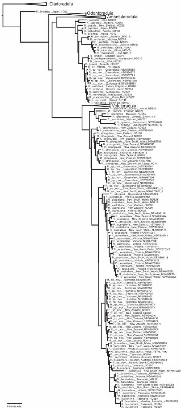
Figure 4. Majority rule phylogram from posterior probability distribution sampled by MrBayes showing the phylogeny of Radula with species named but without morphological groups identified. Branch lengths are proportional to substitution rate.
