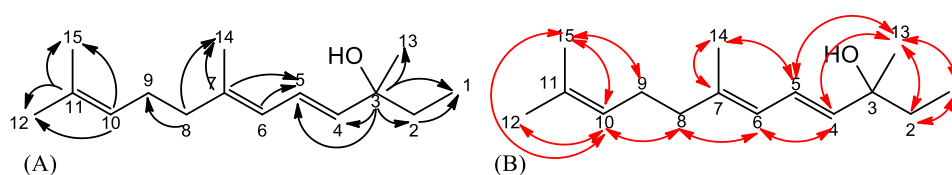
Figure 3. Long range ^{13}\text{C} - ^1\text{H} HMBC (A) and NOE (B) correlations observed in compound 58
