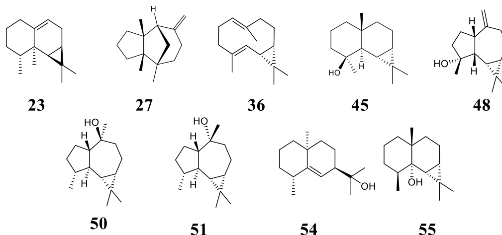
Figure 2. Structures of P. porelloides essential oil components identified by GC-MS and ensured by NMR. (Numbers refers to table 4).
