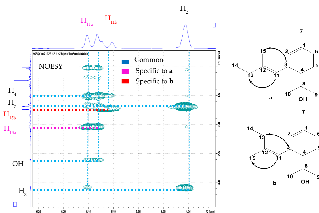
Figure 6. Zoom of NOESY spectrum showing specific correlations used to resolve stereochemistry of the acyclic double bond in 42a , b
