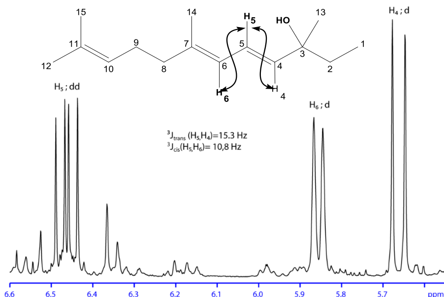
Figure 4. H-H coupling pattern of the ethylenic system of 58
