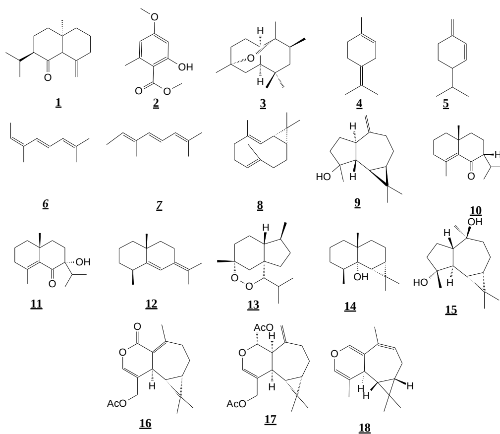
Figure 1. Structures of main components reported from the essential oils of Plagiochila species. (Numbers refers to table 1).
