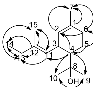
Figure 5. Structure of 42a and schematic representation of HMBC correlations
