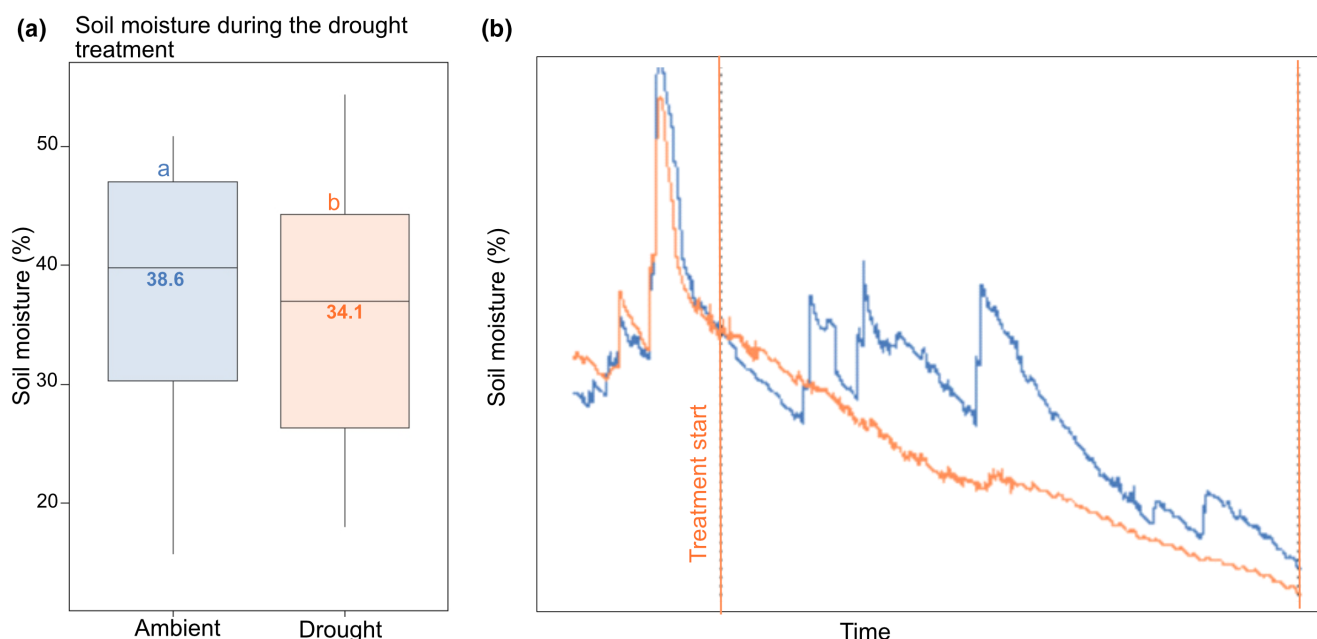
FIGURE 2 (a) Soil moisture during the treatment period in the drought and ambient plots, with the mean soil moisture shown with values in each boxplot ( n=25 ). Different small letters denote a significant difference. (b) An example of the soil moisture change over time for one rainout shelter. The orange line indicates the soil moisture in the drought treatment plot and the blue line indicates the soil moisture in the control plot receiving ambient precipitation.
