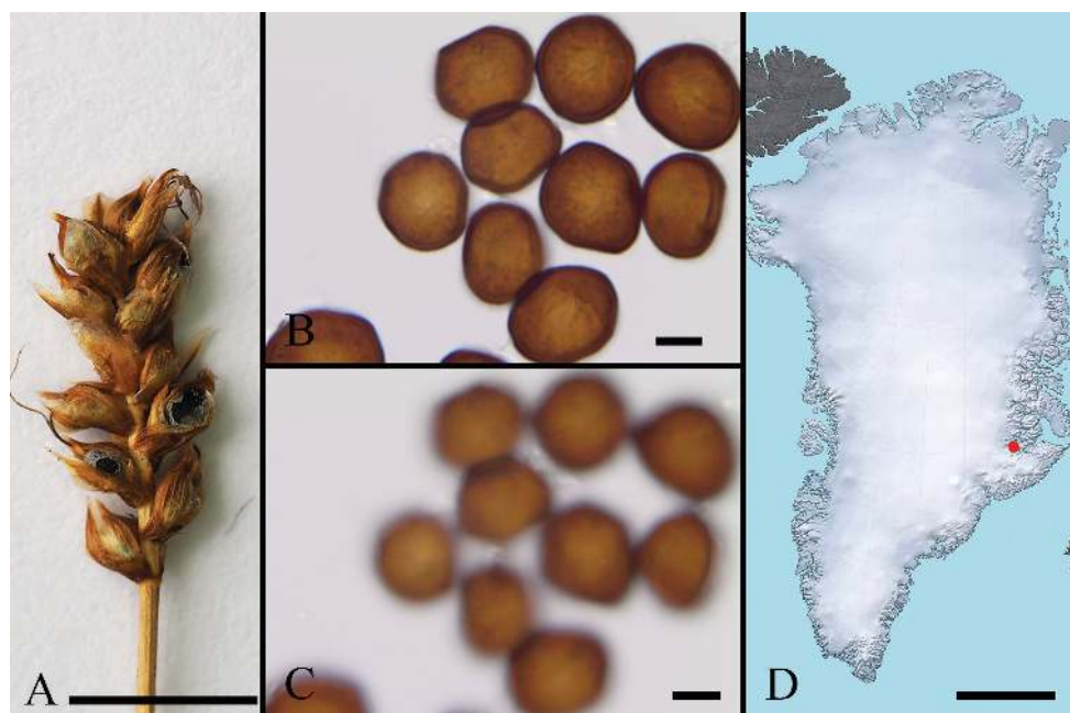
Figure 18. Anthracoidea turfosa on Carex parallela subsp. parallela (S. Lægaard, no. 138, C-Greenland herb., s.n.). A Habit B, C spores in LM, in median and surface view, respectively D distribution map. Scale bars: 0.5 cm ( A ); 10 µm ( B, C ); 500 km ( D ).
