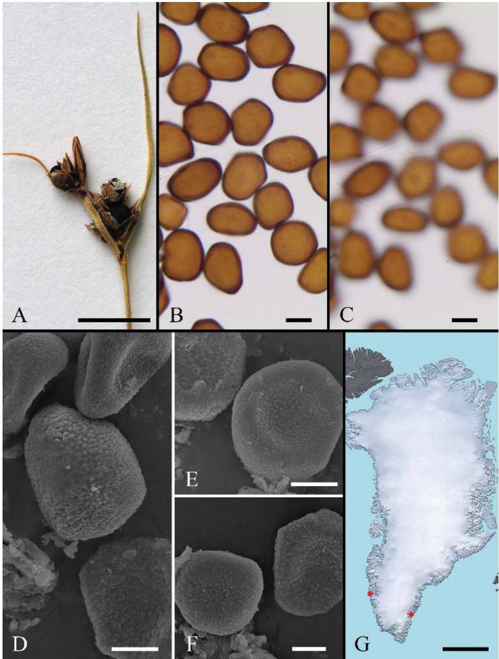
Figure 5. Anthracoidea caricis on Carex deflexa . A Habit (leg. P.F. Scholander, s.n., O, s.n.) B, C spores in LM, in median and surface view, respectively (leg. P.F. Scholander, s.n., O, s.n.) D–F spores in SEM (T.W. Böcher, no. 81, C-Greenland herb., s.n.) G distribution map. Scale bars: 0.5 cm ( A ); 10 µm ( B, C ); 5 µm ( D–F ); 500 km ( G ).
