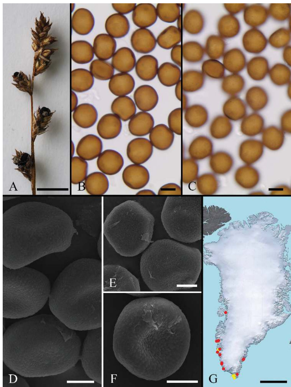
Figure 8. Anthracoidea kariii on Carex brunnescens . A Habit (C-F-107980) B, C spores in LM, in median and surface view, respectively (S. Læggaard, no. 65-3190, C-Greenland herb., s.n.) D–F spores in SEM ( D S. Læggaard, no. 65-3190, C-Greenland herb., s.n.; E H. Andersen & J. Feilberg, no. G.B.U. 4245, C-Greenland herb., s.n.; F A.E. Porsild, no. 8058, C-Greenland herb., s.n.) G distribution map (red circles – on Carex brunnescens ; yellow circles – on a C. canescens ). Scale bars: 0.5 cm ( A ); 10 µm ( B, C ); 5 µm ( D–F ); 500 km ( G ).
