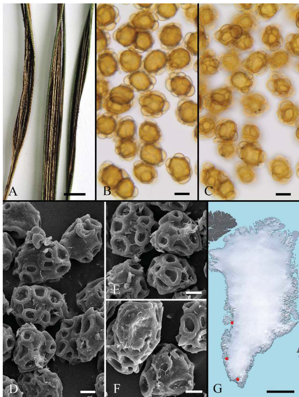
Figure 36. Urocystis agropyri on Leymus arenarius . A Habit (C-F-111316) B, C spore balls in LM (C-F-111316) D–F spore balls in SEM (C-F-102482) G distribution map. Scale bars: 0.5 cm ( A ); 10 µm ( B, C ); 5 µm ( D–F ); 500 km ( G ).
