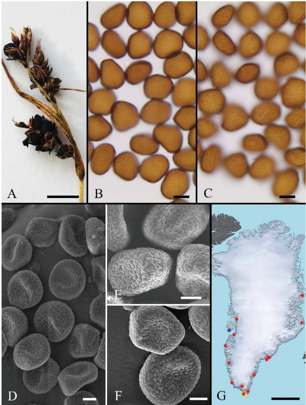
Figure 3. Anthracoidea bigelowii on Carex bigelowii . A habit (C-F-107497) B, C spores in LM, in median and surface view, respectively (C-F-108011) D–F spores in SEM ( D, E 13 Aug 1928, J. Eugenius, s.n., C-Greenland herb., s.n.; F C-F-102524) G distribution map (red circles – on Carex bigelowii ; yellow circles – on hybrids of C. bigelowii ; blue circle – on C. concolor ). Scale bars: 0.5 cm ( A ); 10 \mu m ( B, C ); 5 \mu m ( D–F ); 500 km ( G ).
