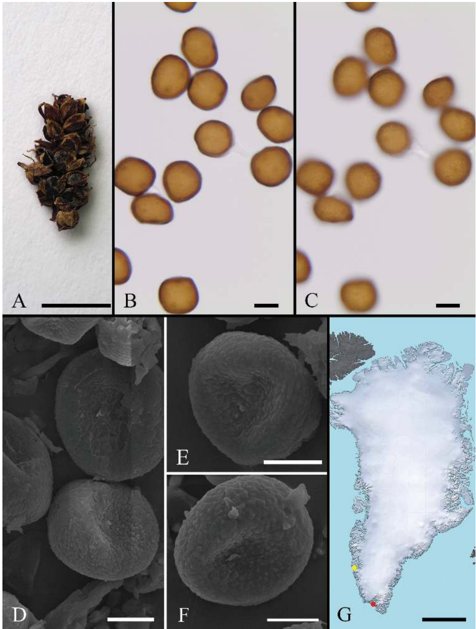
Figure 7. Anthracoidia heterospora on Carex nigra (leg. C.A. Jørgensen, s.n., C-Greenland herb., s.n.). A Habit B, C spores in LM, in median and surface view, respectively D–F spores in SEM G distribution map (red circle – on Carex nigra ; yellow circle – on a hybrid of C. bigelowii ). Scale bars: 0.5 cm ( A ); 10 \mu m ( B, C ); 5 \mu m ( D–F ); 500 km ( G ).
