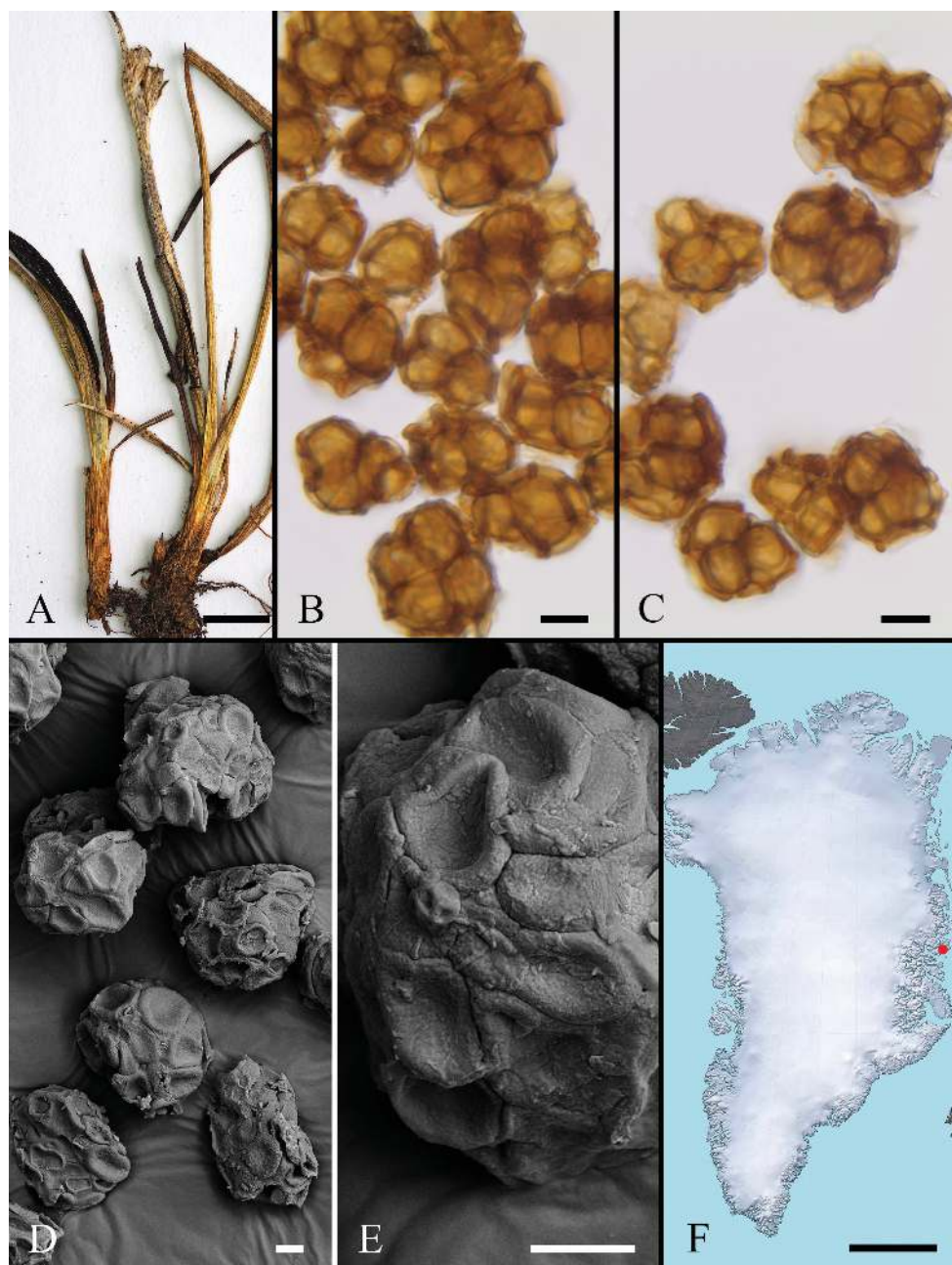
Figure 40. Urocystis tothi on Juncus biglumis (leg. A. Hagen, s.n., O. s.n.). A Habit B, C spore balls in LM D, E spore balls in SEM F distribution map. Scale bars: 0.5 cm ( A ); 10 µm ( B, C ); 5 µm ( D, E ); 500 km ( F ).
