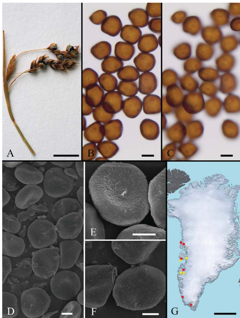
Figure 4. Anthracoidea capillaris on Carex capillaris (A–C, E, F) and C. boecheriana (D). A Habit (S. Frederiksen & L.B. Jørgensen, no. 68-1699, C-Greenland herb., s.n.) B, C spores in LM, in median and surface view, respectively (V. Dalgaard, no. 86-396, C-Greenland herb., s.n.) D–F spores in SEM ( D 20 Jul 1926, leg. M.P. Porsild, s.n., C-Greenland herb., s.n.; E S. Frederiksen & L.B. Jørgensen, no. 68-1699, C-Greenland herb., s.n.; F 19 Jul 1939, leg. M.P. Porsild, s.n., C-Greenland herb., s.n.) G distribution map (red circles – on Carex capillaris ; yellow circles – on C. boecheriana ). Scale bars: 0.5 cm (A); 10 µm (B, C); 5 µm (D–F); 500 km (G).
