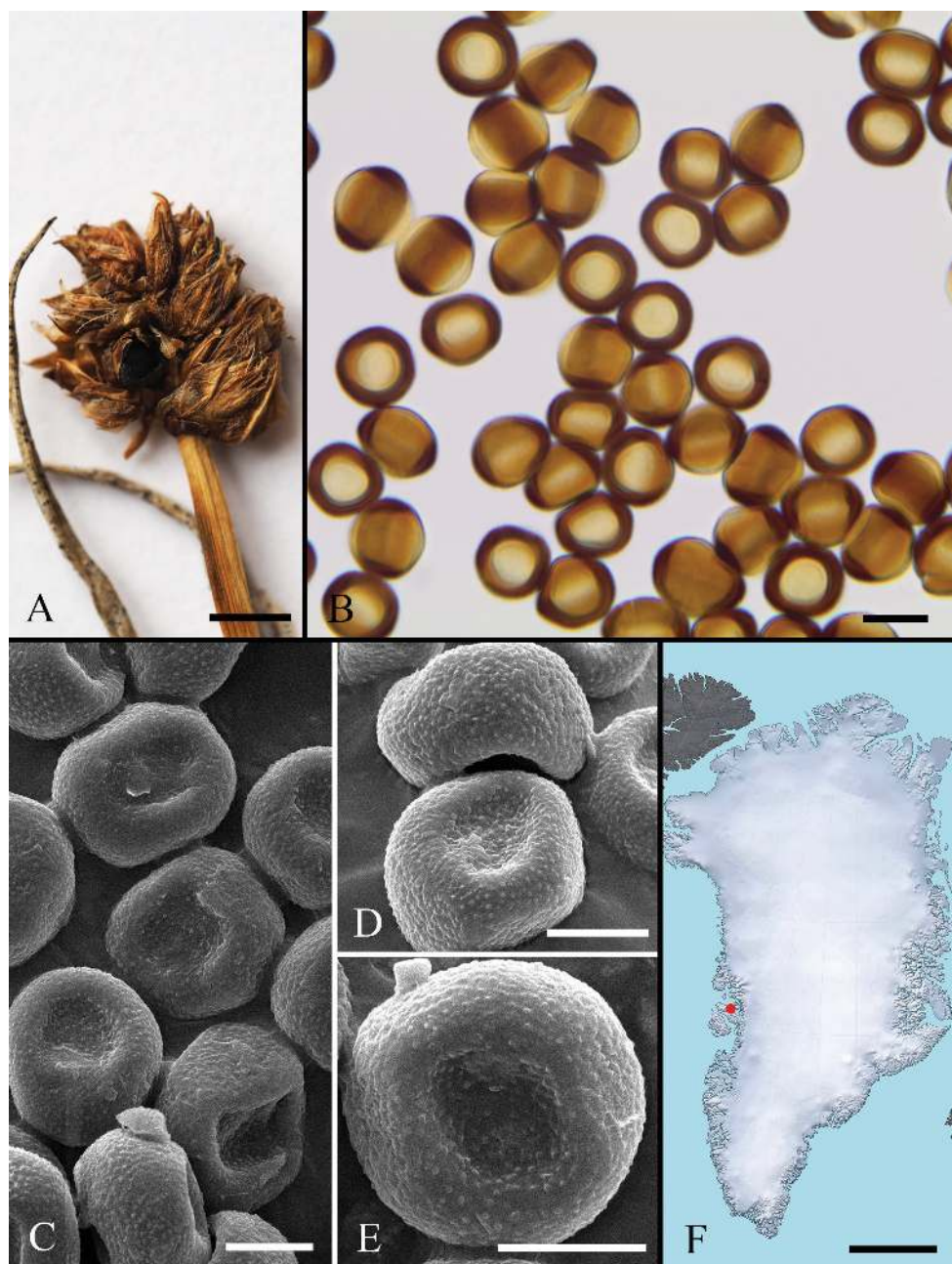
Figure 30. Planetella lironis on Carex maritima (T. Sørensen, no. 9196, C-Greenland herb., s.n.). A Habit B spores in LM C–E spores in SEM F distribution map. D, E reproduced, with permission, from Denchev & Denchev 2018. Scale bars: 0.5 cm ( A ); 10 µm ( B ); 5 µm ( C–E ); 500 km ( F ).
