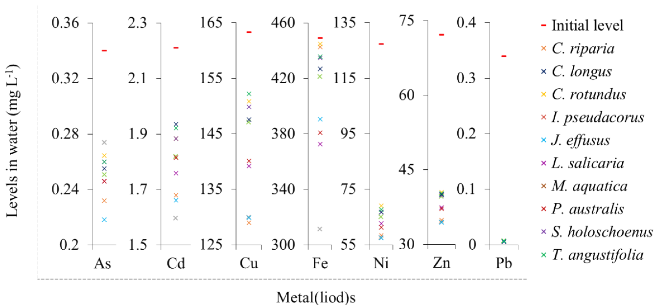
Figure 3 Concentrations of metal(loid)s in groundwater on the 15 th day of exposure for the respective plant treatment. The x-axis represents the different metal(loid)s; the y-axis the respective metal(loid) concentrations in mg L -1 . The red line indicates the initial concentration at the start of the experiment (0 day), while the different coloured cross signs indicate the residual metal(loid) concentration in the groundwater for the respective plants.
