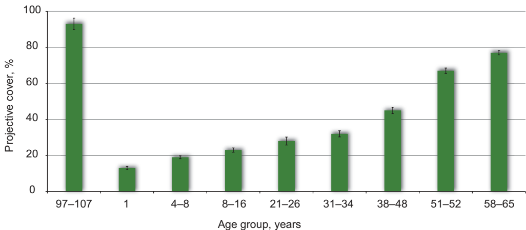
Fig. 6. The dynamics of the projective cover of Rhododendron luteum undergrowth in forest plantations established after main clear-cutting in the moist fairly infertile pine site type ( B_3 )
