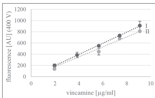
Fig. 2: Fluorescence of dilution series of vincamine in 0.1 M H 2 SO 4 (pH 1, I) and 0.01 M H 2 SO 4 (pH 1.9, II)
