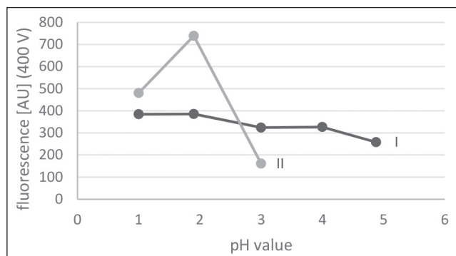
Fig. 1: pH dependence of ion pairing of vincamine [4 µg/ml] (I) and protopine [4 µg/ml] (II) with sodium-9,10-dimethoxy-anthracene-sulfonate [200 µg/ml] – fluorometrically measured in the organic solvent.
