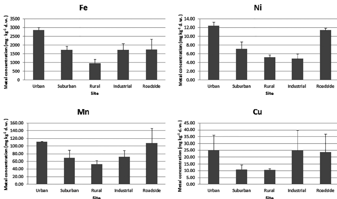
Fig. 2. Fe, Cu, Mn and Ni mean concentrations in aboveground parts of Polygonum aviculare from different sites in the studied area (mg kg -1 dry weight \pm SD) in the city of Kragujevac.
