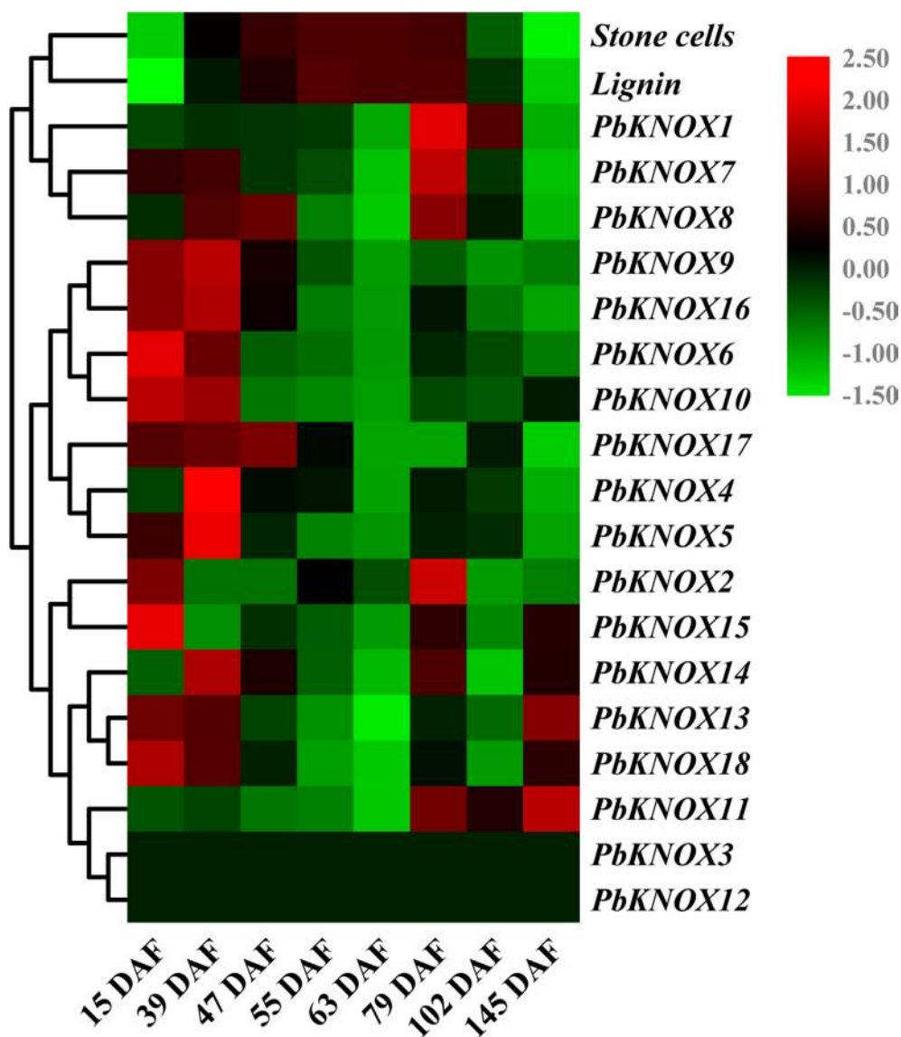
FIGURE 6 | Hierarchical clustering analysis of stone cell/lignin levels, and transcription levels of PbKNOX s in pear fruits at different developmental stages. The qRT-PCR results are presented in a heatmap, and the expression trends were clustered. Stone cells: percentage of stone cell content in pear pulp (%). Lignin: percentage of lignin content in pear pulp (%).
