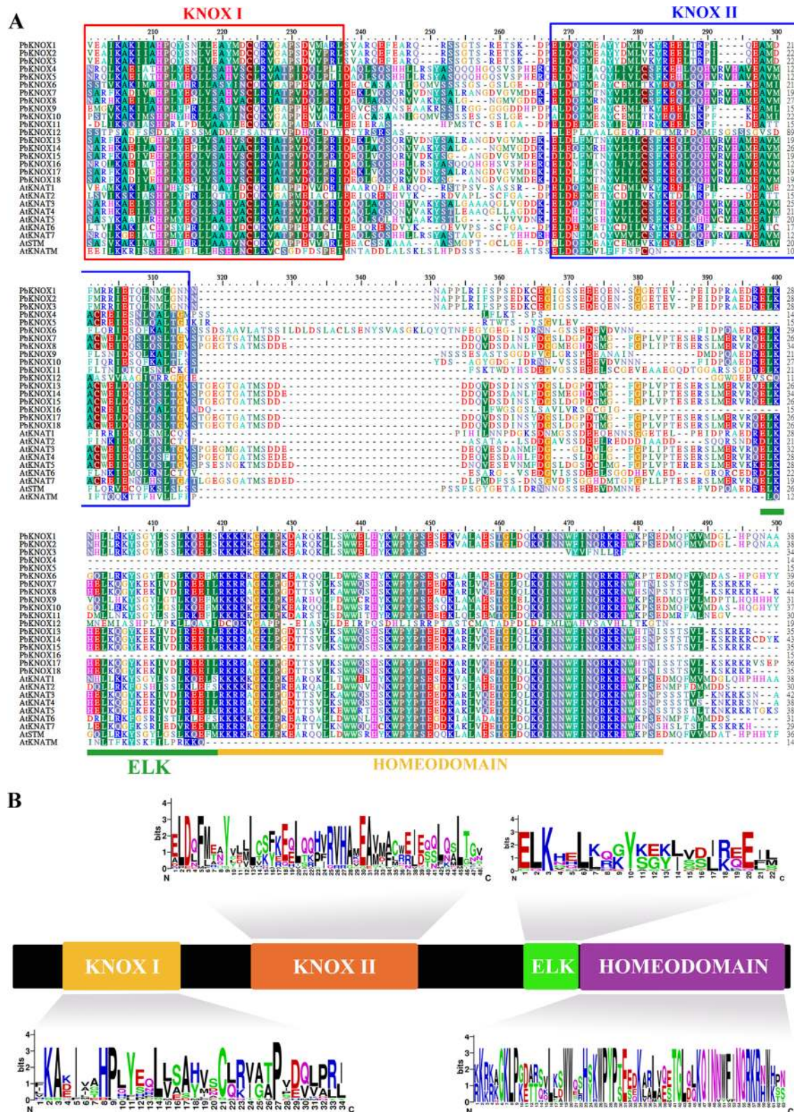
FIGURE 1 | Multiple sequence alignment and domain compositions of PbKNOX proteins. (A) Multiple sequence alignment of KNOX proteins from various plants. (B) The distribution and composition of the characteristic motifs of PbKNOX proteins. The bit score represents the information content for each position in the sequence. The logo consists of stacks of symbols, one stack for each position in the sequence. The overall height of the stack indicates the sequence conservation at that position, while the height of symbols within the stack indicates the relative frequency of each amino acid at that position.
