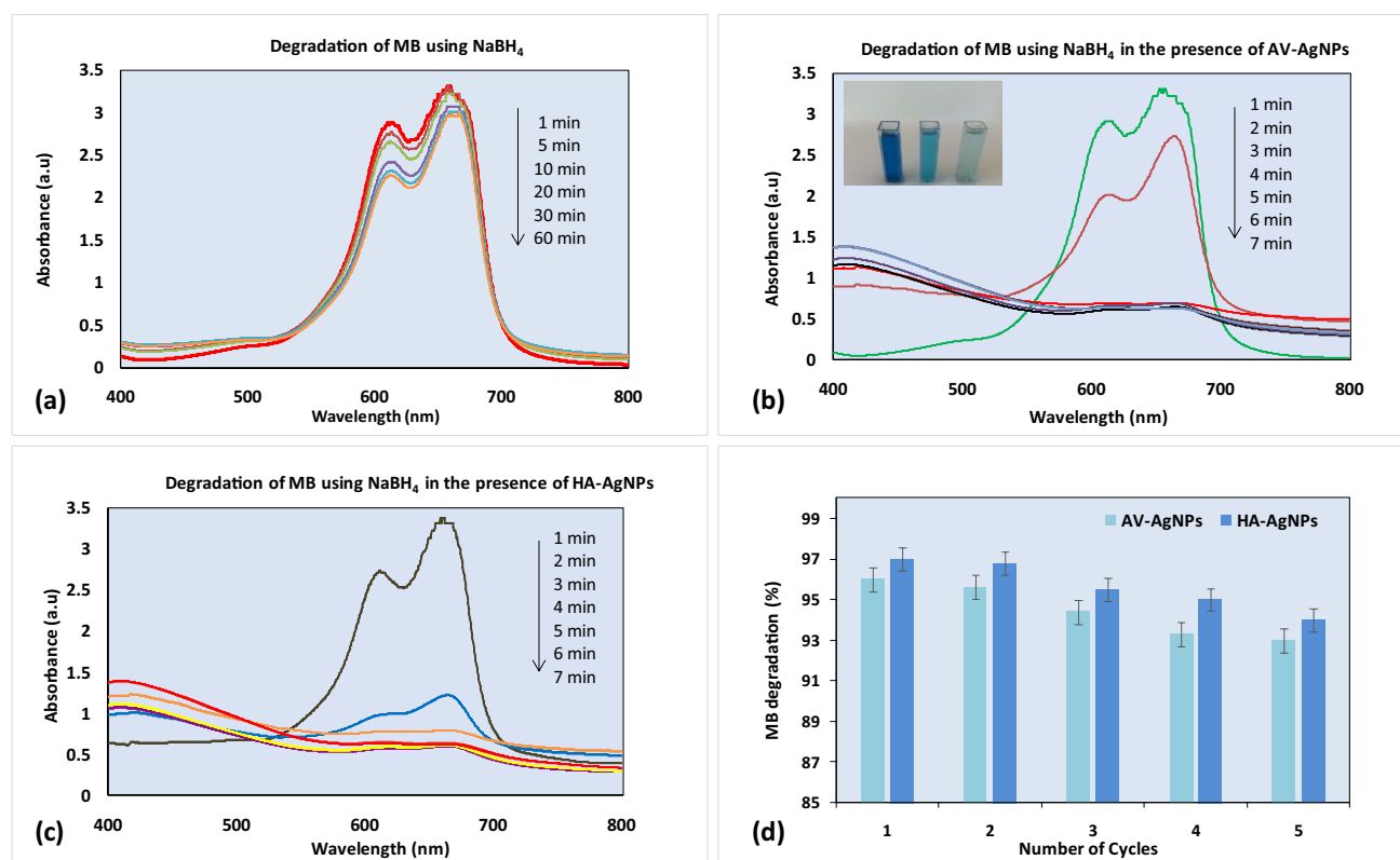
Fig. 7 MB degradation using \text{NaBH}_4 in the absence of any AgNPs (a), degradation of MB using \text{NaBH}_4 in the presence of AV-AgNPs and HA-AgNPs (b, c), number of cycles for AV-AgNPs and HA-AgNPs (d)
