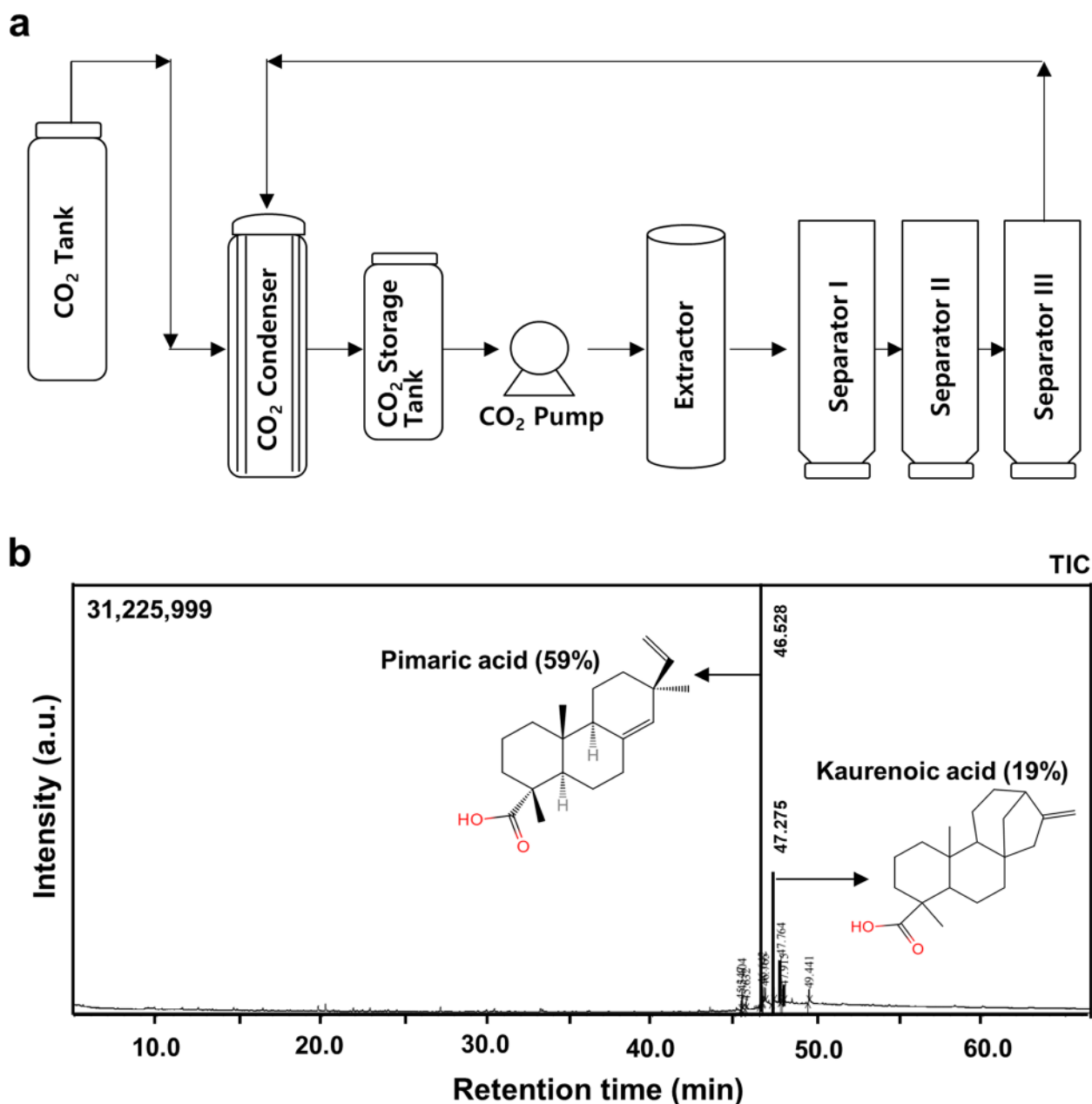
Fig. 1 Schematic representation of the supercritical extraction apparatus and GC-MS chromatogram for A. sessiliflorus Harms extract using supercritical CO 2
