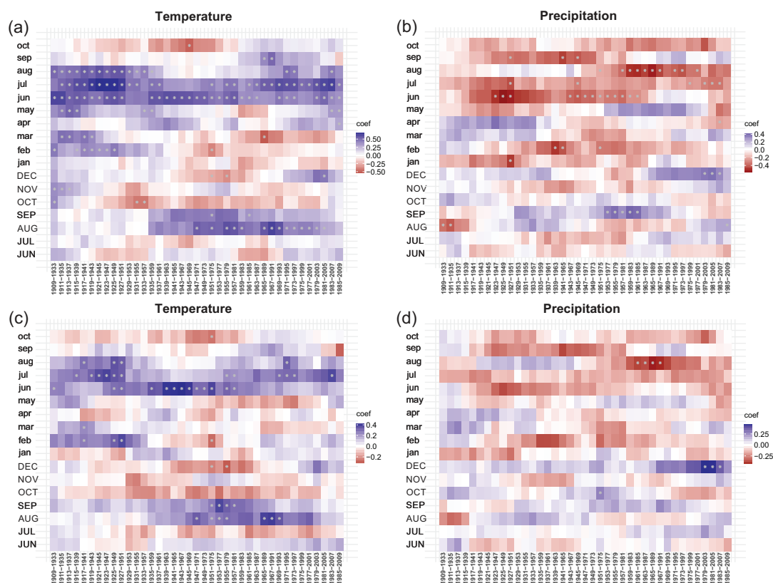
Figure 4. Moving correlation coefficients (a) and (b) and response function coefficients (c) and (d), calculated over 25 year windows with 2 year offsets over the period 1907–2009, between the standardized Cassiope tetragona shoot length chronology and mean monthly temperatures as well as monthly precipitation sums, as modelled for the Pika valley, Kluane Region, Yukon Territory, Canada. Asterisks (*) indicate significant coefficients. Abbreviations of months from the year of growth are in lowercase letters and those of the previous year are given in capitals.
