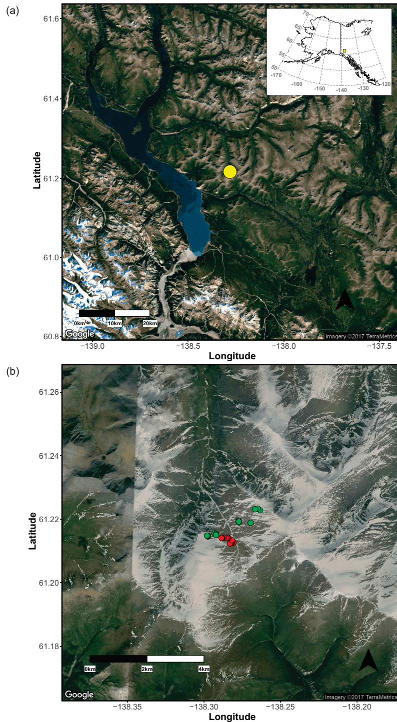
Figure 1. Location of the Kluane Region in the Yukon Territory northwest Canada indicated with a yellow square on the inset map and the location of the Pika valley (yellow circle) northwest of Kluane Lake (a). Satellite image map of the Pika valley and adjacent areas (b); sampling spots of Cassiope tetragona are marked with red dots; sampling locations of Salix pulchra are indicated with green dots.
