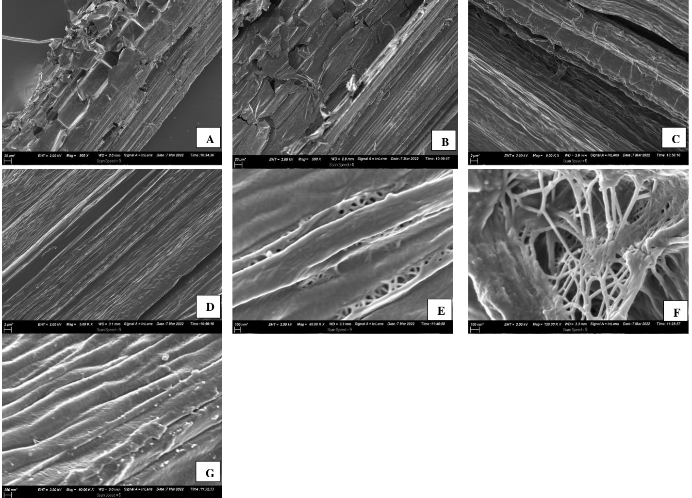
Figure I: SEM images for yellow thatching grass; (a) for untreated sample ;( b) for dewaxed sample; (c) for pulped sample; (d) for bleached sample; (e) for CNF1 ; (f) for CNF 3 and (g) for CNF 5.6 respectively.
