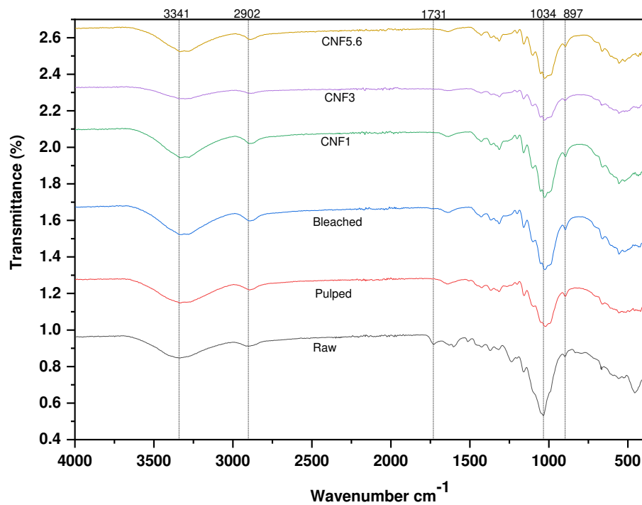
Figure III: FTIR Spectra of raw, bleached, pulped and acid-hydrolyzed samples
