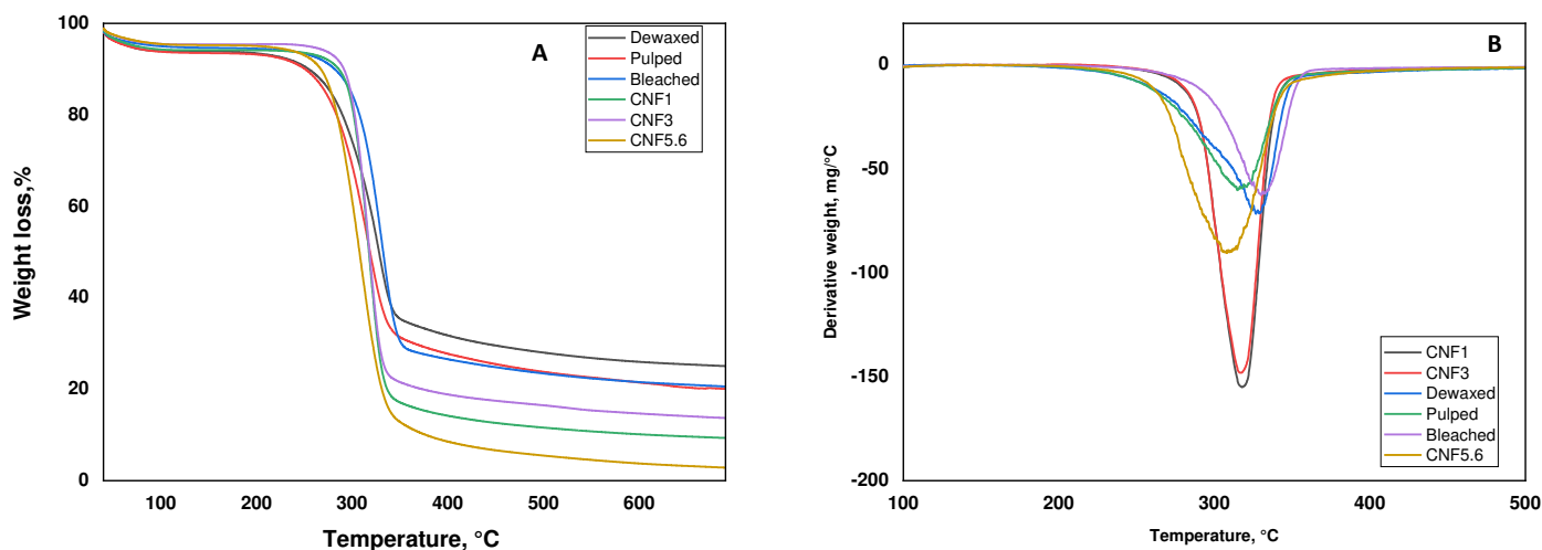
Figure V: (a) TGA and (b) DTG curves for samples
