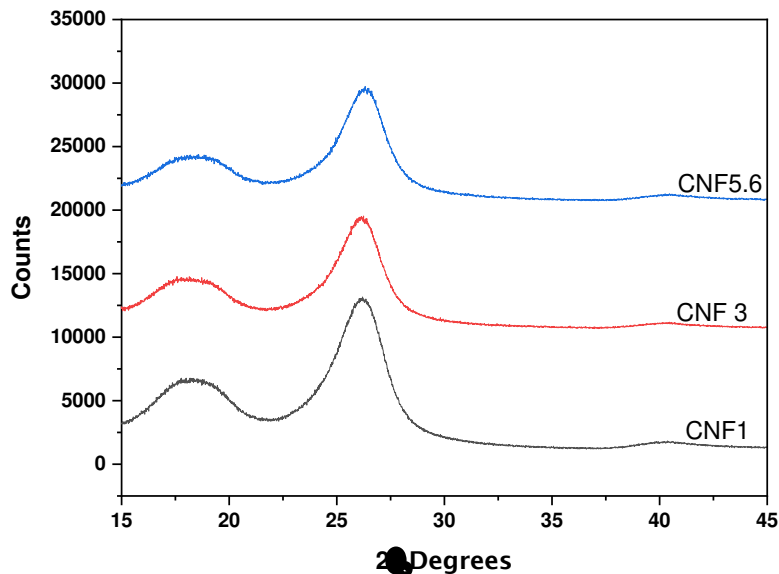
Figure IV: XRD patterns of acid-hydrolyzed CNF samples
