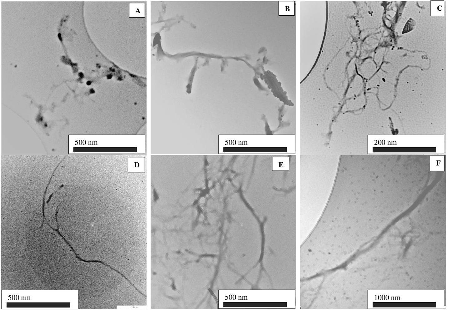
Figure II: TEM images of yellow thatching grass; a (Raw sample); b (De-waxed); c (Bleached); d (CNF1); e (CNF 3); f (CNF 5.6) respectively.
