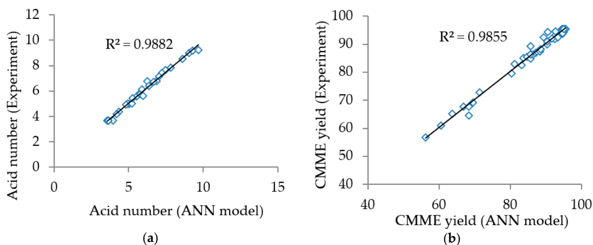
Figure 2. Experimental values versus values predicted by the ANN model integrated with ant colony optimization (ACO) for (a) acid-catalyzed esterification (acid number) and (b) base-catalyzed transesterification [ C. manghas methyl ester (CMME) yield].
