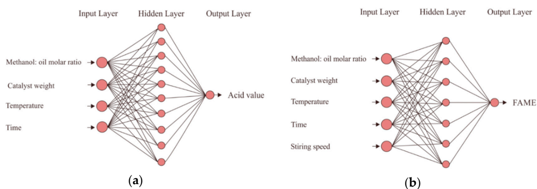
Figure 1. Neural network architecture for (a) acid-catalyzed esterification and (b) base-catalyzed transesterification.
