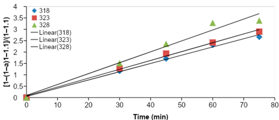
Figure 5. Plot of [1 - (1 - a)^{1-1.1}] / (1 - 1.1) versus time.
