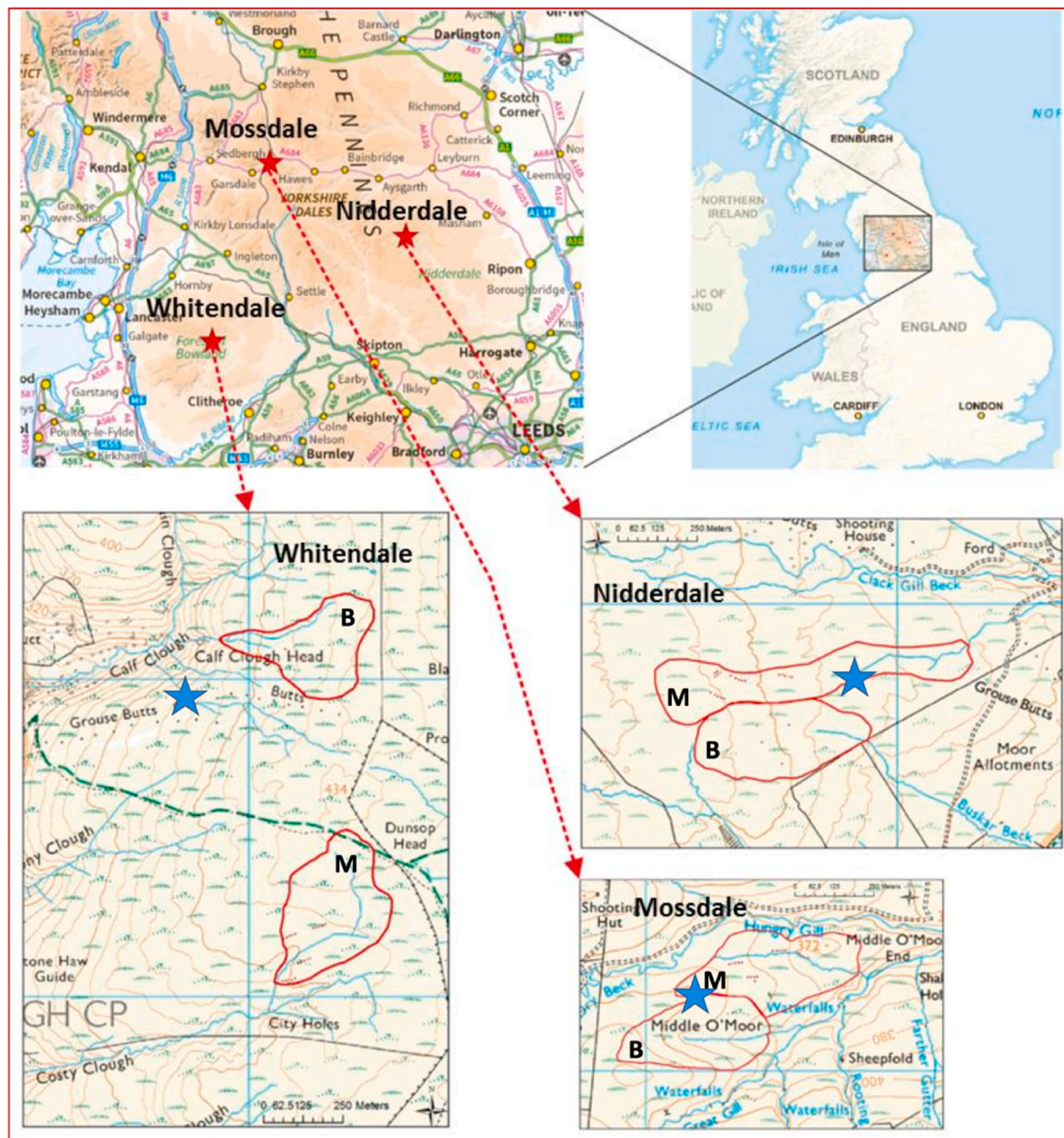
Fig. 1. Location of the three study sites in northern England ( top maps , red stars). The catchment boundaries (thick red lines) with the burnt (B) and cut/mown (M) catchments are detailed in the lower maps for Whitendale, Mossdale and Nidderdale with weather station locations indicated by a blue star. Source: MiniScale® [TIFF geospatial data], Scale 1:1,000,000, Tiles: GB, Updated: December 3, 2015, Ordnance Survey (GB), Using: EDINA Digimap Ordnance Survey Service, http://d igimap.edina.ac.uk , Downloaded: 2016-09-09 14:35:01.73. Note the central stream within each sub-catchment (map taken from Heinemeyer et al., 2019b).
