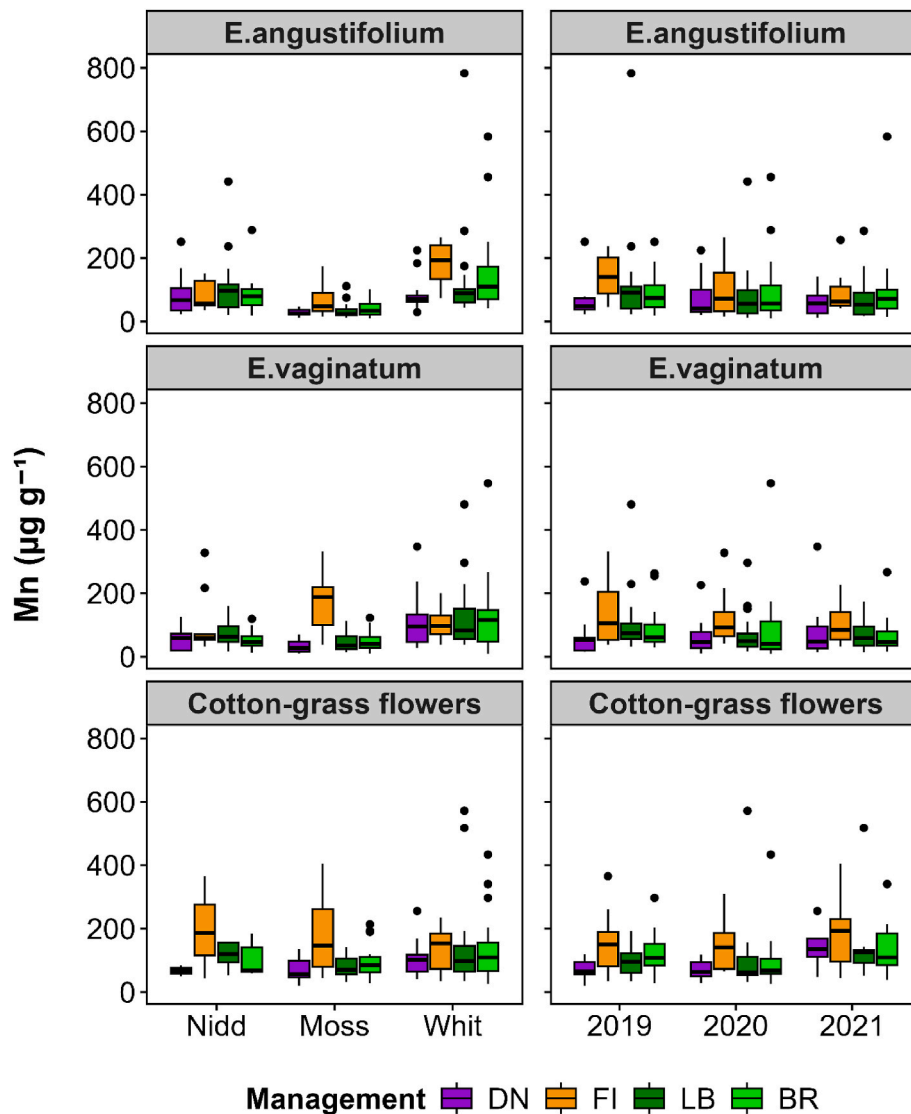
Fig. 4. Elemental concentration of manganese (Mn) in sedge (i.e., cotton-grass; Eriophorum angustifolium and E. vaginatum ) leaves and ( E. spp. ) flowers, either across the three sites for Nidderdale (Nidd), Mossdale (Moss) and Whitendale (Whit), or for different years (2019–2021) for the four management treatments of either unmanaged 'do nothing' (DN), fire 'burnt' (FI) and cut with either left brash (LB) or brash removal (BR). Significant differences are shown in Table 2A,B.
