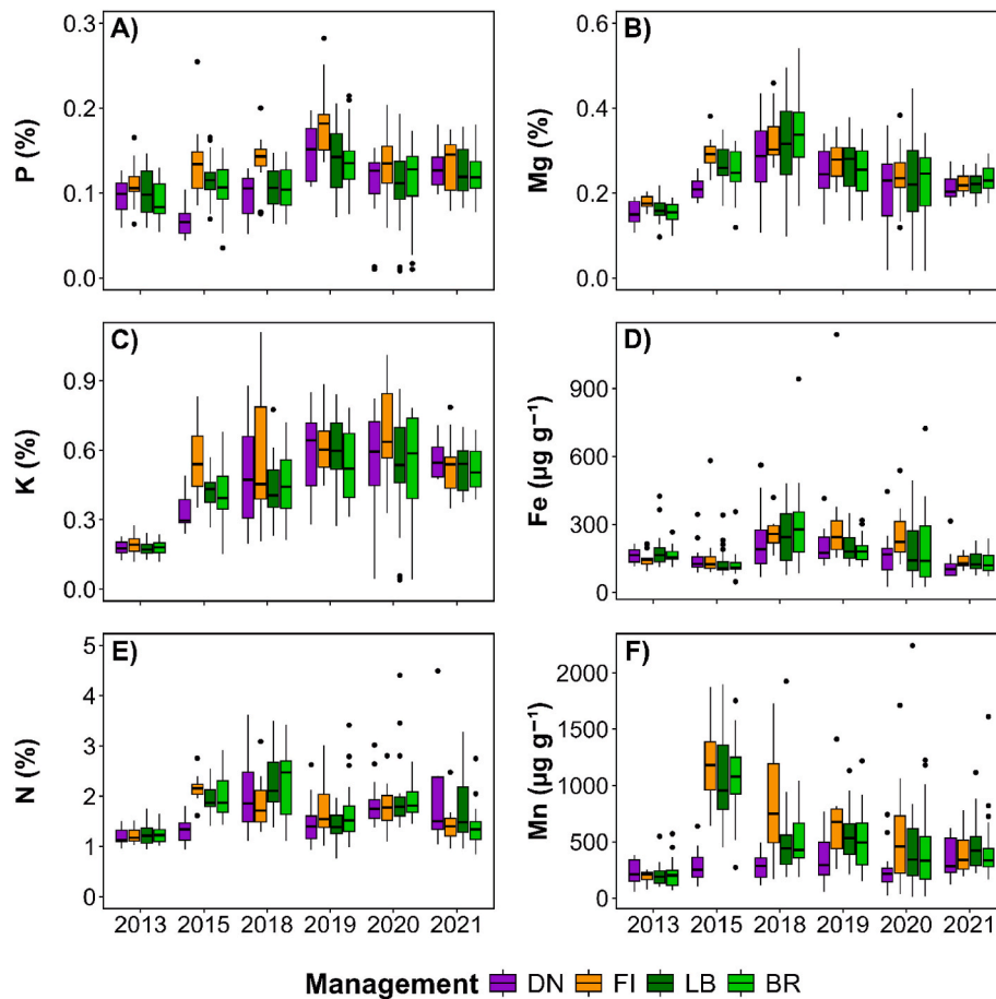
Fig. 3. Elemental content (either as percentage or concentration) in heather shoots combined for all three sites over time for A) phosphorus (P), B) magnesium (Mg), C) potassium (K), D) iron (Fe), E) nitrogen (N) and F) manganese (Mn), for the four management treatments of either unmanaged 'do nothing' (DN), fire 'burnt' (FI) and cut with either left brash (LB) or brash removal (BR). Significant differences are shown in Table 1A,B.
