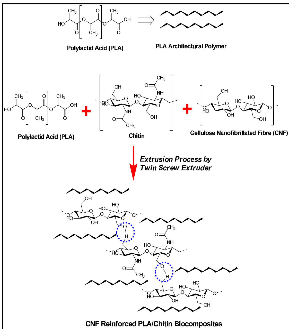
Figure 8. Schematic diagram of Possible chemical interaction between PLA, chitosan, and CNF
