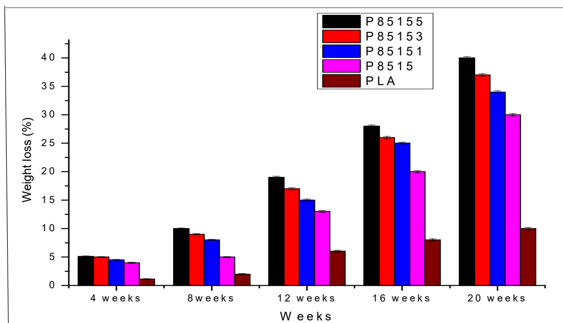
Figure 2. Biodegradation weight loss percentage of neat PLA, P8515, P85151, P85153, and P85155.
