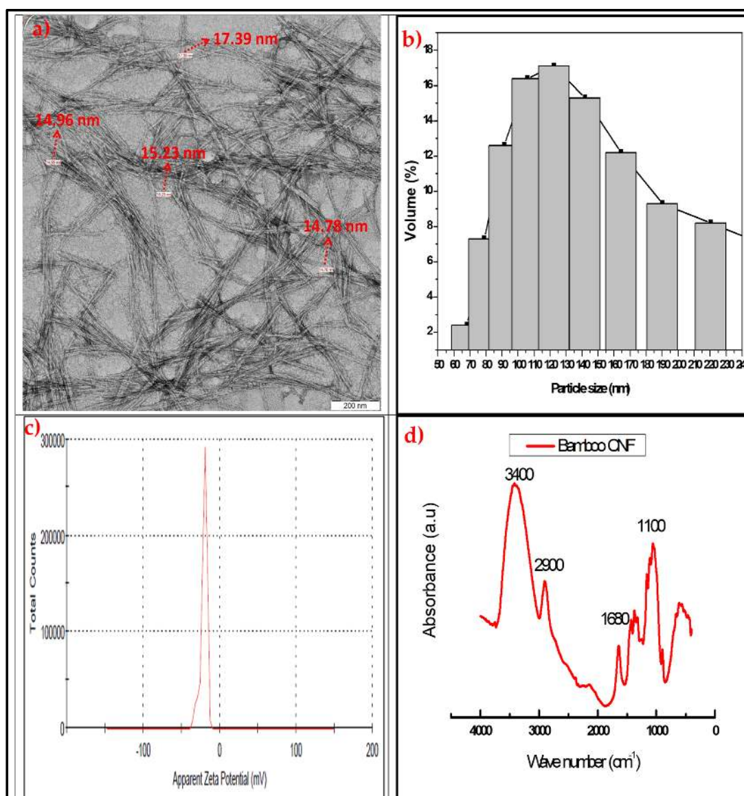
Figure 1. (a) TEM, (b) particle size analysis, (c) zeta potential, and (d) FT-IR analysis of Schizostachyum brachycladum bamboo cellulose nanofibre.
