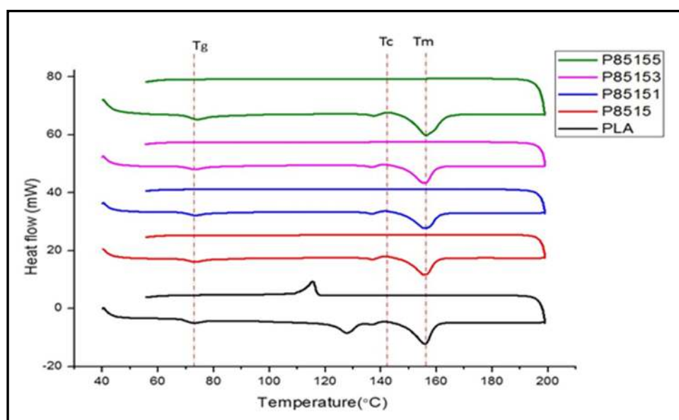
Figure 5. Differential scanning calorimetry for neat PLA, P8515, P85151, P85153, and P85155 biocomposites.
