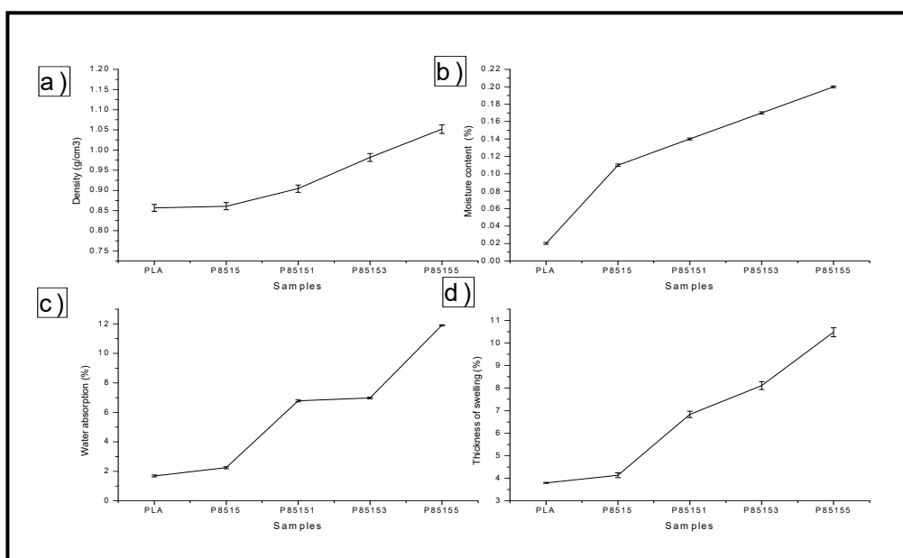
Figure 9. Physical properties (a) Density, (b) Moisture content, (c) water absorption, (d) Thickness swelling for neat PLA, P8515, P85151, P85153, and P85155 biocomposites.
