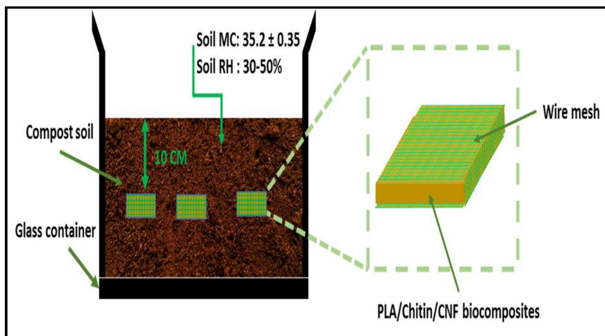
Figure 10. Schematic drawing of soil burial test set up for molecular biodegradation of neat PLA and biocomposite.
