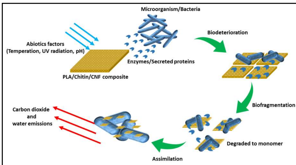
Figure 3. Schematic diagram of molecular enzymatic degradation process in soil burial test.
