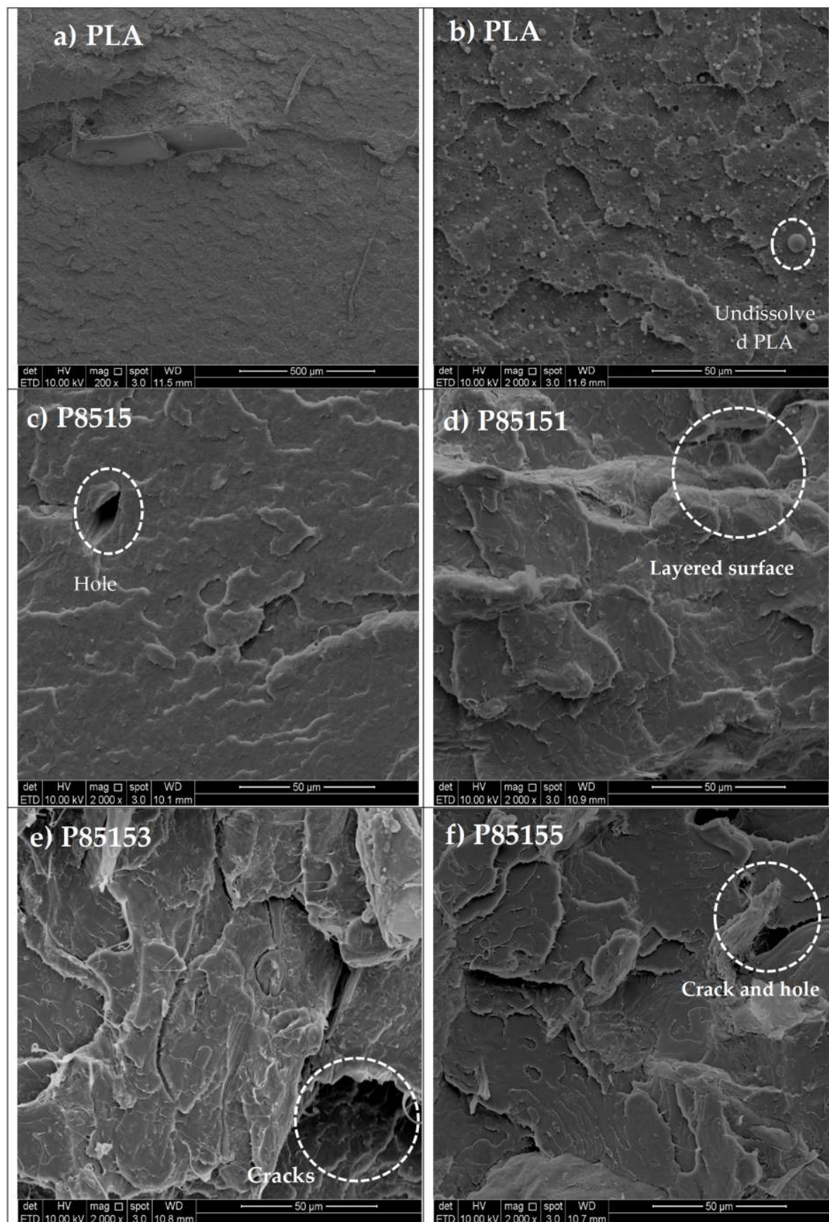
Figure 7. Tensile fractured surface SEM images for neat PLA, P8515, P85151, P85153, and P85155 biocomposites.
