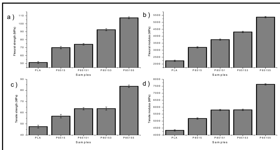
Figure 6. Mechanical properties (a) Flexural strength, (b) Flexural modulus, (c) Tensile strength, (d) Tensile modulus for neat PLA, P8515, P85151, P85153, and P85155 biocomposites.
