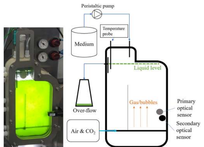
Fig. 1. The assembled 400 mL Algaemist-S flat-panel photobioreactor. The flask indicated as “over-flow” in the diagram collects the outflow from the reactor, which was recorded daily. The secondary optical sensor continuously measures the transmitted light, which controls the turbidity by adding fresh cultivation medium by activating a peristaltic pump. Light-blocking covers were temporarily removed in this picture.
