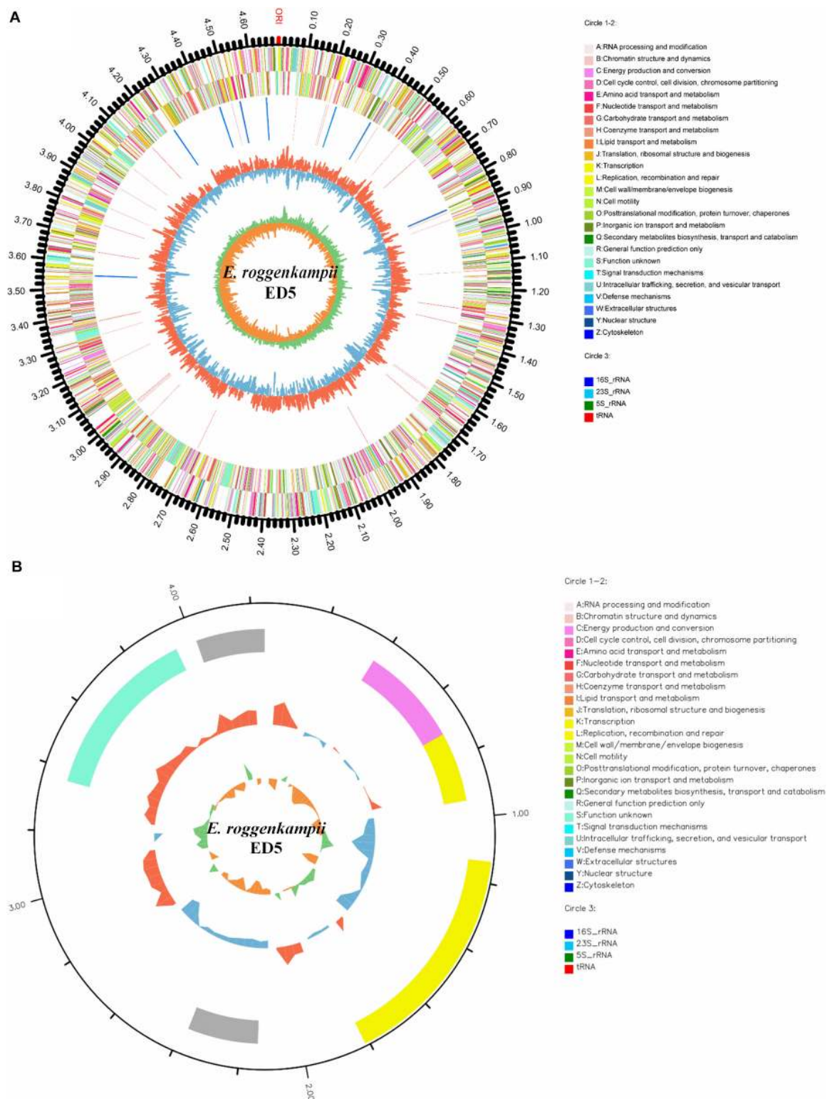
FIGURE 5 | Circular representation of chromosome and plasmid of endophytic nitrogen-fixing E. roggkampii ED5 strain isolated from sugarcane root. The inner and innermost rings display the GC content and skew. ORI; the origin of replication in chromosome map. (A,B) : A–Z, respectively, show the functional classification of the CDS genes in the chromosome and plasmid with the colors of the COG database and circle 3; different colors show different RNA types.
