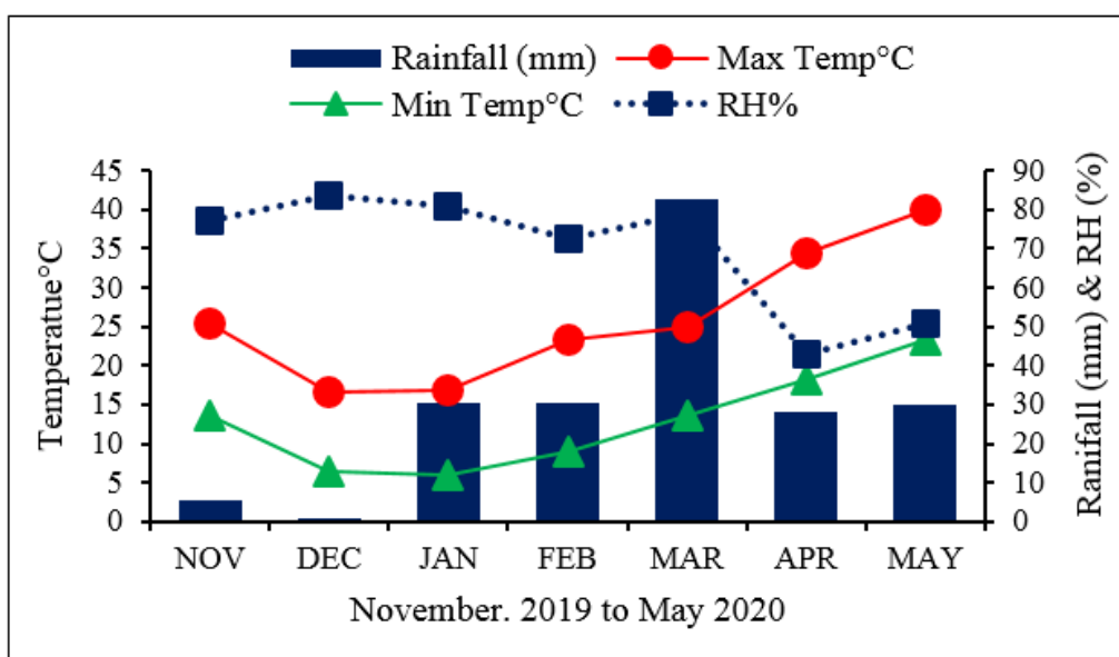
Figure 1: Weather Attributes of Experimental Site during November, 2019 to May 2020
