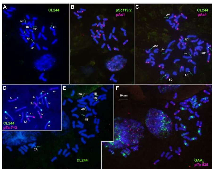
FIGURE 3 Localization of CL244 (green) repeat on Ae. crassa , 4x ( A,B ), Ae. crassa , 6x ( C ), Th. bessarabicum ( D ), and common wheat ( E,F ) chromosomes. Chromosomes are identified using pAs1 ( B,C , red), pTa-713 ( D , red) or GAA n ( F , green) and pTa-535 ( F , red). Chromosomes carrying CL244 signals are indicated. Scale bar, 10 μm.
