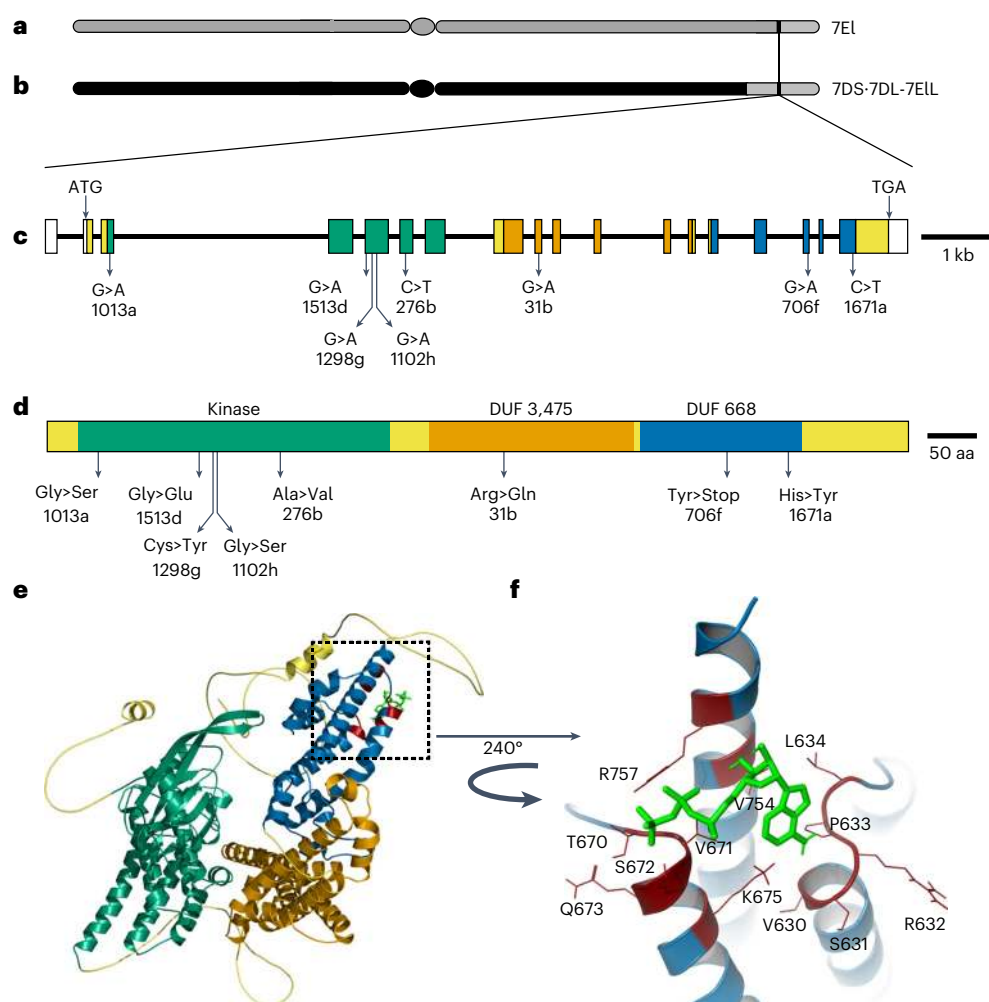
Fig. 1 | Sr43 encodes a protein kinase fused to two DUFs. a , Th. elongatum chromosome 7. b , Schematic diagram of the wheat- Thinopyrum translocation chromosome. c , Identified EMS mutations along the predicted Sr43 gene model. d , Schematic diagram of Sr43 , showing predicted domains and amino acid changes induced by the EMS mutations. e , Three-dimensional model of Sr43 , as predicted by AlphaFold. Green, kinase; orange and blue, DUF domains; yellow,
