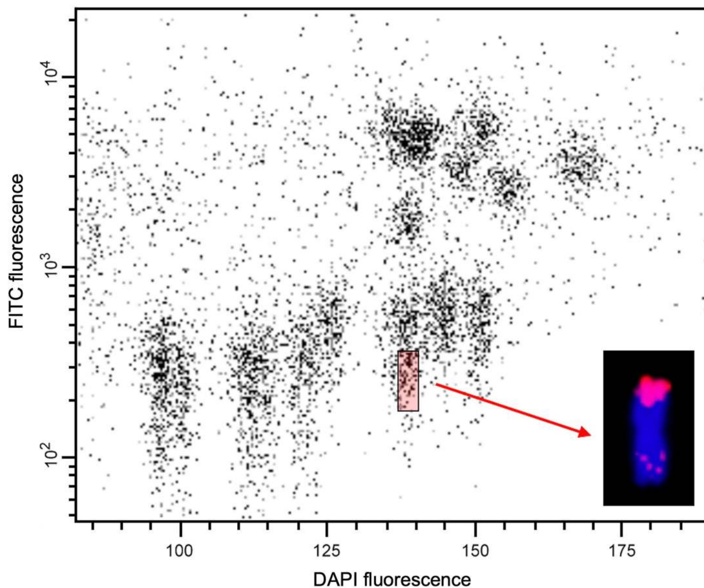
Extended Data Fig. 1 | Bivariate flow karyotype of mitotic metaphase chromosomes isolated from the wheat- Th. elongatum 7D/7eL2 translocation line carrying the Sr43 resistance gene. DAPI (x-axis) vs. FITC (y-axis) dot plot was obtained after the analysis of DAPI-stained chromosome suspensions labeled by FISHIS with FITC-conjugated probes for GAA and ACG microsatellites. The
