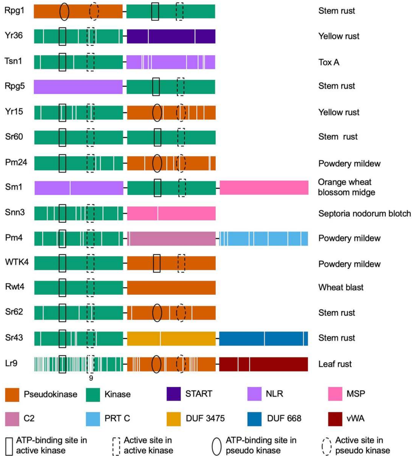
Extended Data Fig. 7 | Schematic diagrams of Triticeae kinase fusion proteins with disease resistance function. The ATP-binding and active sites of the kinases are indicated by boxes and circles in the active and pseudo kinases, respectively, as determined by Interpro scanning, homology searching in AlphaFold-derived 3D models and/or BLAST. White bars indicate loss-of-function missense mutations obtained from EMS mutant screens. Eight mutations in the linker domains are not shown. The proteins are organized from top to bottom by date of publication: Rpg1, Yr36, Tsn1, Rpg5, Yr15, Sr60, Pm24, Sm1, Snn3, Pm4 (encoded by splice version 2), WTK4, Rwt4, Sr62 (refs. 9–21), Sr43 (this study)
