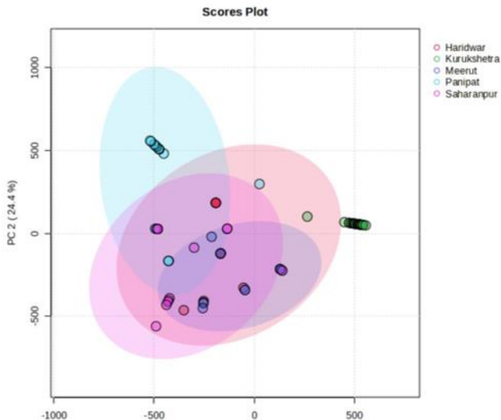
Figure 3: Principal components analysis
