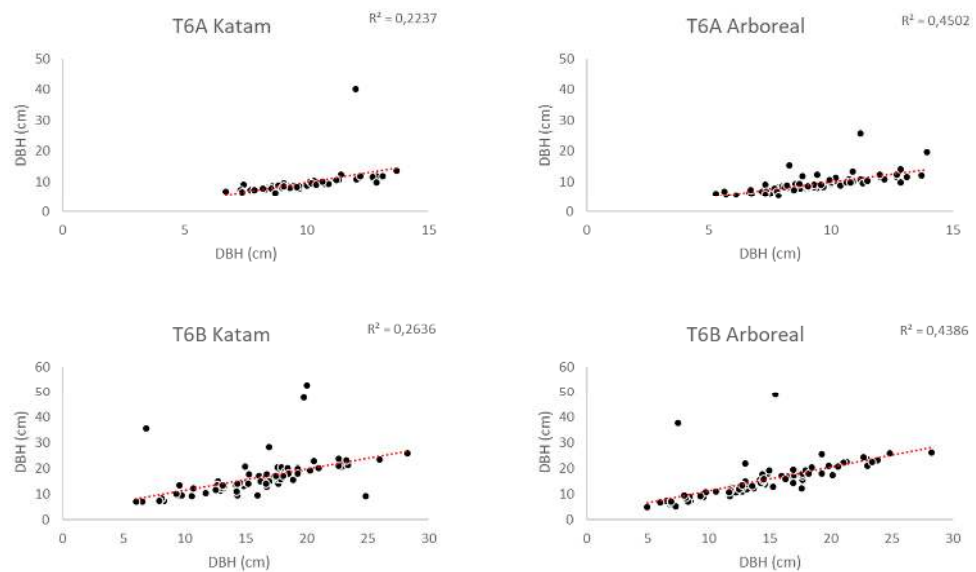
Figure 9. Scatter plot of the diameter values evaluated by the traditional method (XX axis) and by the Katam and Arboreal apps for typologies T6A and T6B (eucalyptus plantation in coppice with at least two stems per tree).
