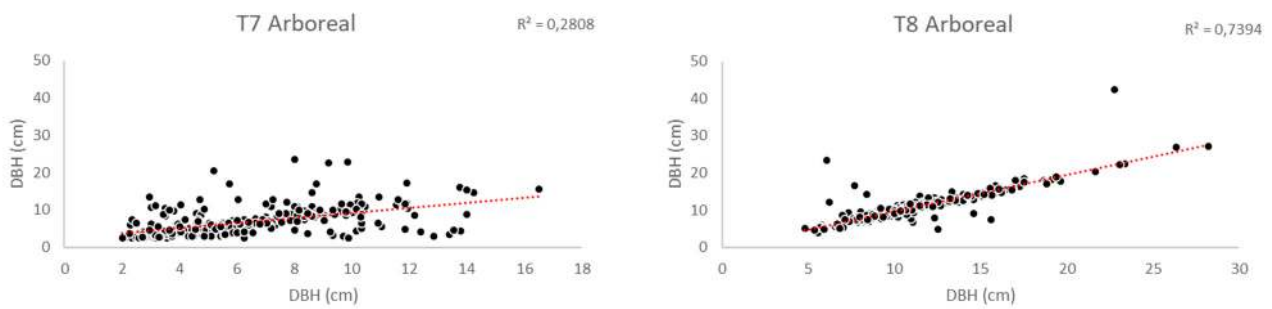
Figure 10. Scatter plot of the diameter values evaluated by the traditional method (XX axis) by the Arboreal app in typologies T7 and T8 (naturally regenerating young pine with variation in age and number of trees per hectare).
