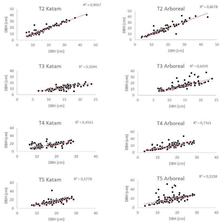
Figure 8. Scatter plot of the diameter values evaluated by the traditional method (XX axis) and by the Katam and Arboreal apps for typologies T2, T3, T4, and T5 (adult eucalyptus plantations with approximately 20 m in height with variation in the slope of the land and in the density of the under-cover vegetation).
