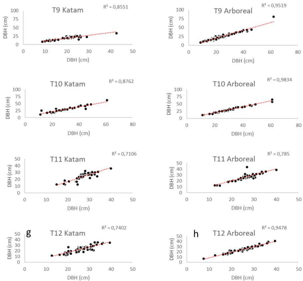
Figure 11. Scatter plot of the diameter values evaluated by the traditional method (XX axis) and by the Katam and Arboreal apps for typologies T9, T10, T11, and T12 (adult planted pine forest with variation in their under-cover vegetation density and slope).
