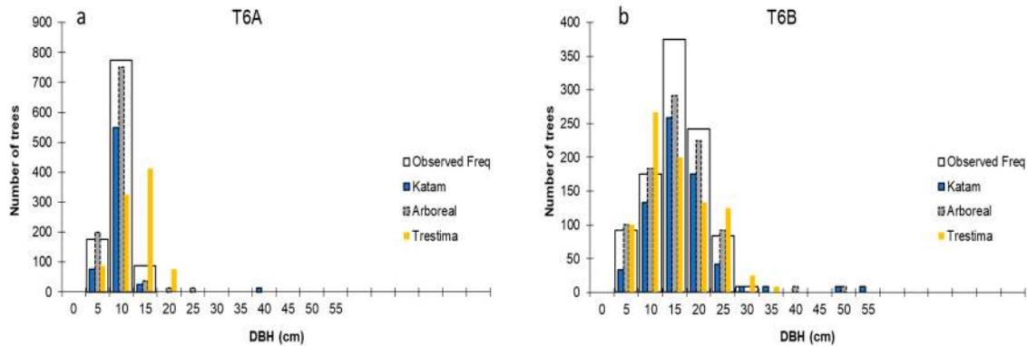
Figure 15. Diameter distributions for types T6A (a) and T6B (b) concerning the Eucalyptus plantation in coppice with at least two poles per tree.
