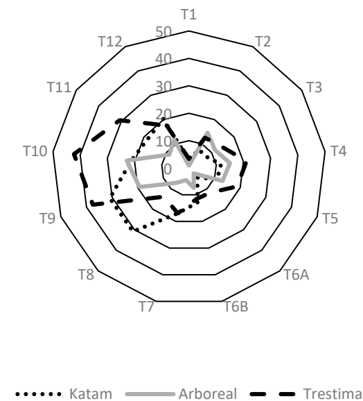
Figure 18. Representation of the Error Index ( \text{m}^2/\text{ha} ) by typology in a radar chart.
