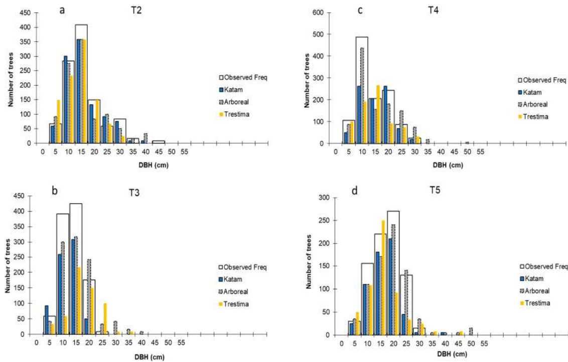
Figure 14. Diameter distributions for types T2 (a), T3 (b), T4 (c), and T5 (d) concerning the adult Eucalyptus plantations with approximately 20 m in height with variations in the slope of the terrain and in the density of the under-cover vegetation.
