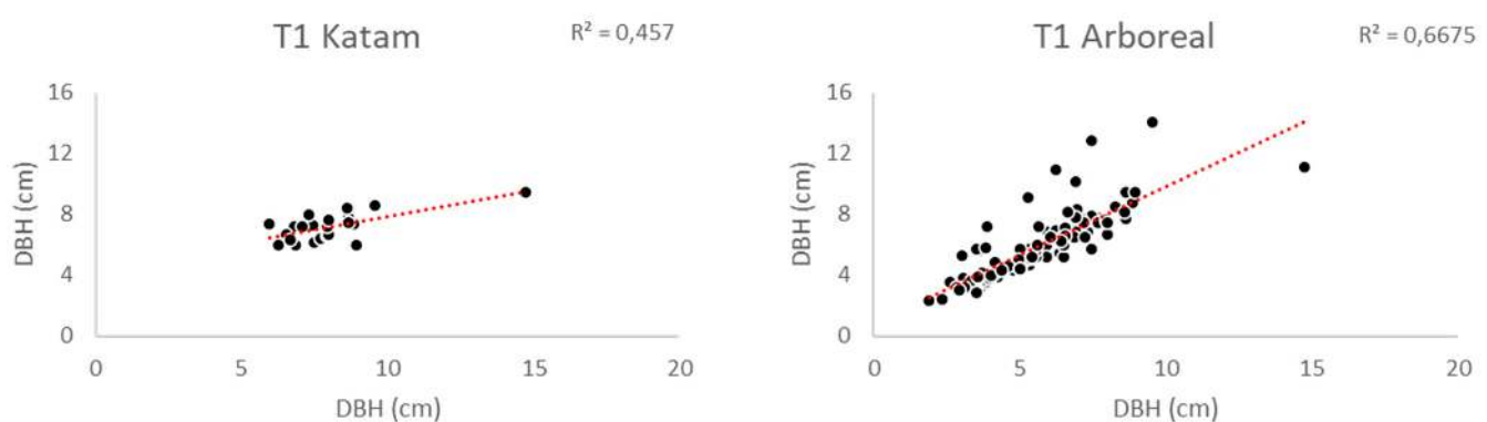
Figure 7. Scatter plot of the diameter values evaluated by the traditional method (X axis) and by the Katam and Arboreal applications for the T1 typology (young high-forest eucalyptus plantations up to 2 m high).
