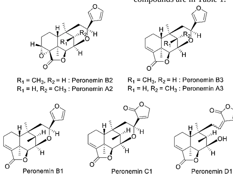
Figure 1. Peronemin structure and derivatives
