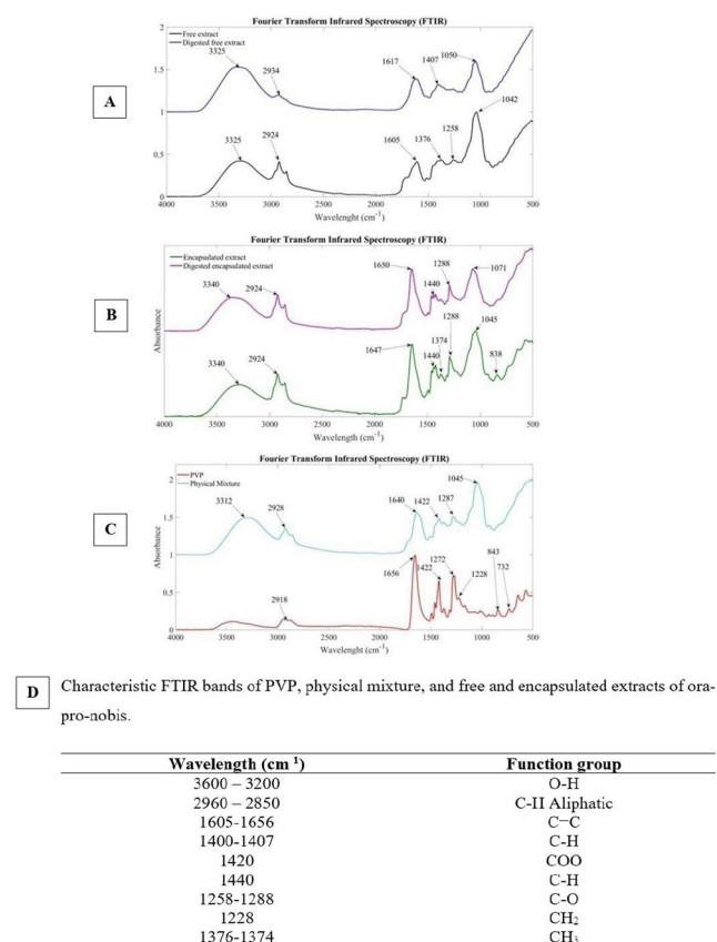
Fig. 1 FTIR spectra of free and PVP-encapsulated ora-pro-nobis extracts and related samples obtained in the wavenumber range of 4000–400 cm -1 . (A) Spectra of the undigested free extract and digested free extract. (B) Spectra of the undigested PVP-encapsulated extract and digested encapsulated extract. (C) Spectra of the encapsulating agent (PVP) and the physical mixture containing 62% free extract and 38% PVP. (D) Characteristic FTIR bands of PVP, physical mixture, and free and encapsulated ora-pro-nobis extracts
