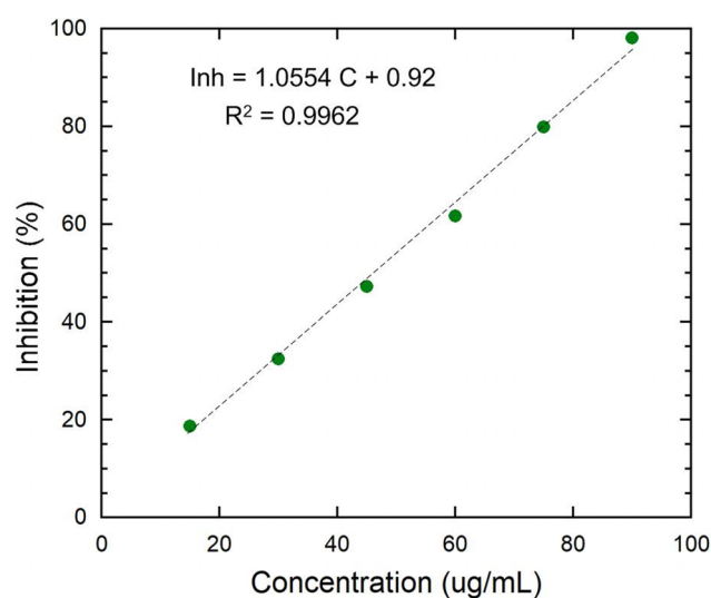
Fig. 9 Antioxidant activity of SiO 2 -NPs synthesized using Tridax procumbens
