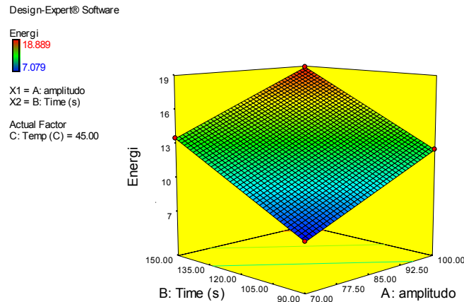
Figure 1. Response surface plot effect of time and amplitude of sonication on energy input
