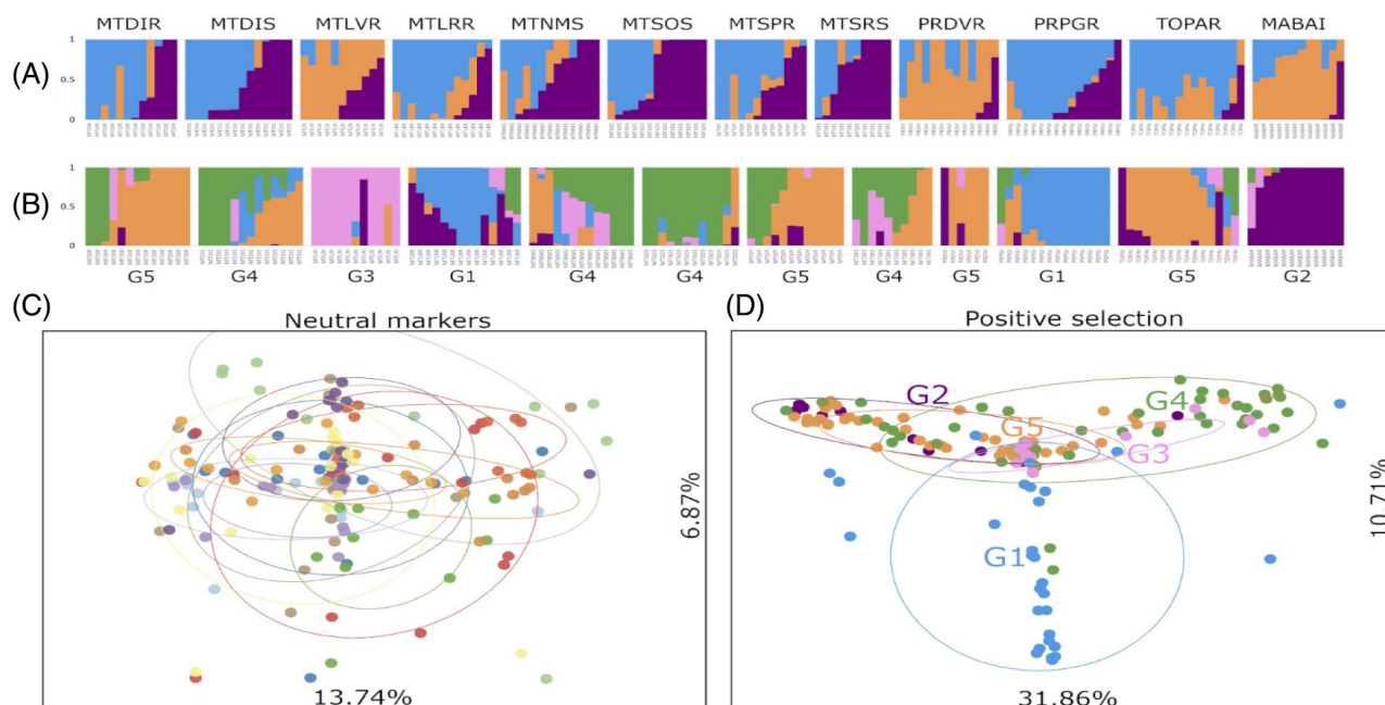
Figure 5. ADMIXTURE and principal component analysis (PCA) of 12 Digitaria insularis populations. ADMIXTURE analysis was performed using 1134 neutral single nucleotide polymorphisms (SNPs) with K = 3 (A), and 687 SNPs under positive selection and K = 5 (B). PCA with neutral SNPs (C) and SNPs under positive selection (D) were also performed. Populations were divided into five groups (G1–G5) for the analyses with SNPs under positive selection.
