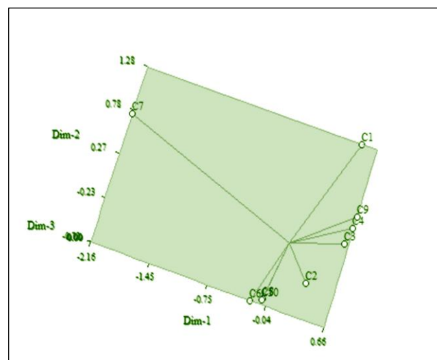
Figure 5: Based on Euclidian distance, principal component analysis (PCA)-3D graphical association between the indicator plants treated with Parthenium leaf, stem, and flower with methanol extract
