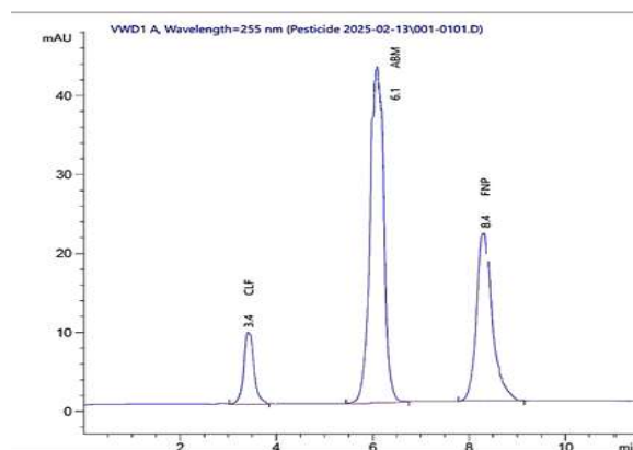
Figure 3: RP-HPLC chromatogram of the mixture: 0.40 \mu\text{g/mL} CLF, 1.00 \mu\text{g/mL} ABM, and 1.20 \mu\text{g/mL} FNP using AN: 5 mM AA buffer (70: 30, v/v), pH adjusted to 4.00, Flow rate 1.20 mL/min, and UV detection at 255 nm.
