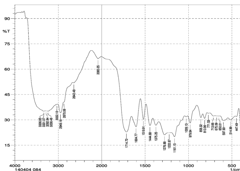
Figure 2. FT-IR spectrum of isolated compounds
