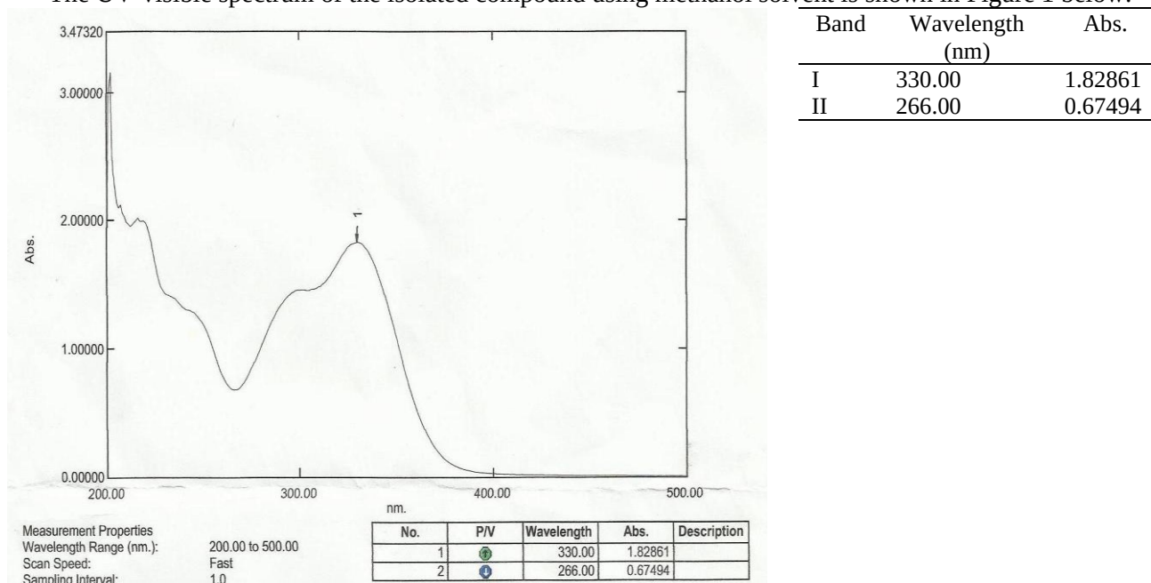
Figure 1 UV-visible spectrum of isolation result compound
