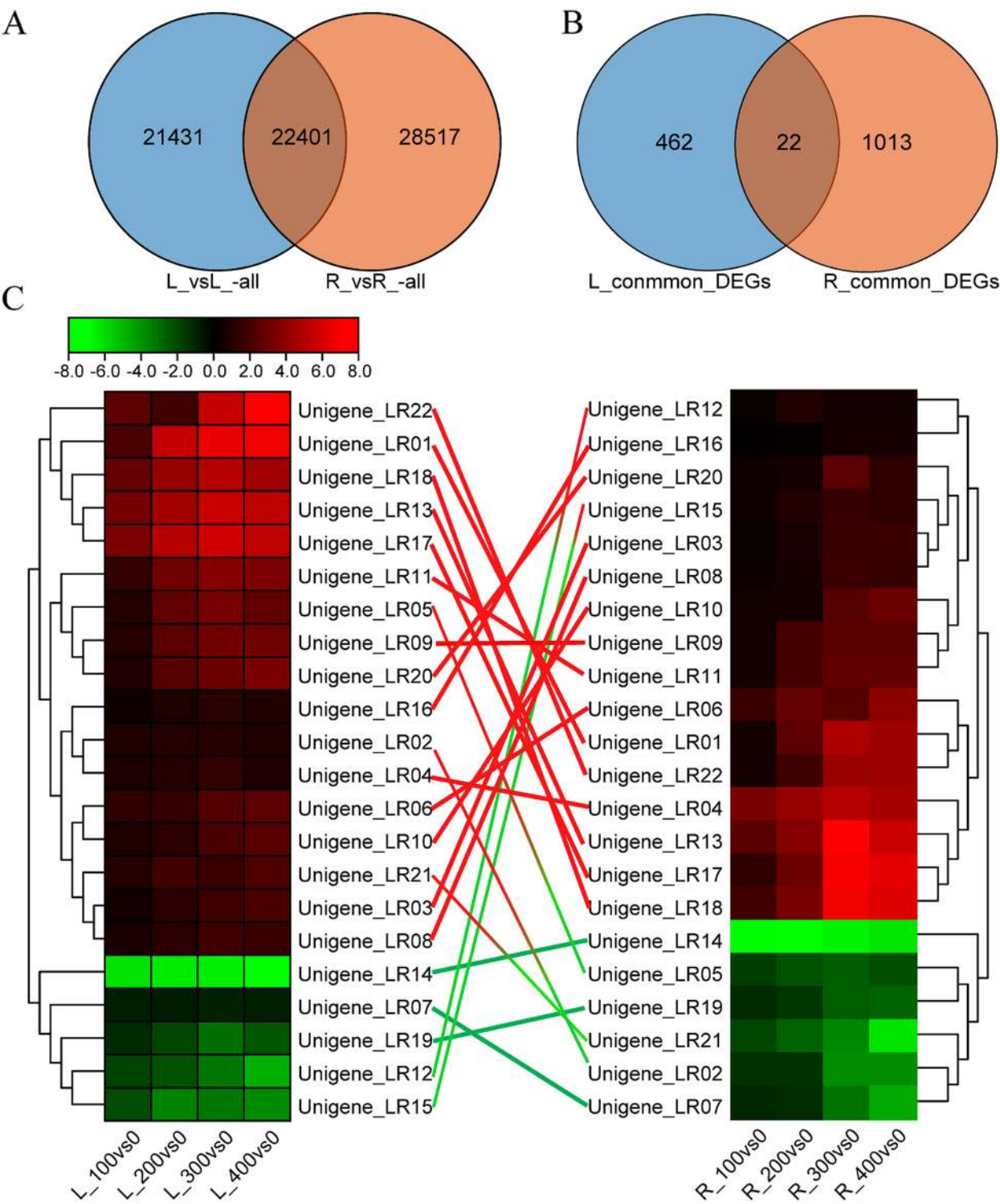
Fig. 8 Co-expressed genes in the leaves and roots. A Venn diagram of all DEGs in the leaves and roots. B Venn diagram of DEGs under different salt concentrations. C Expression patterns of genes co-expressed in the leaves (left) and roots (right). The red connecting lines indicate genes showing up-regulated expression in both leaves and roots; green connecting lines indicate genes showing down-regulated expression in both leaves and roots; gradient lines (red-green) indicate genes showing up-regulated expression in leaves but down-regulated expression in roots; gradient lines (green-red) indicate genes showing down-regulated expression in leaves but up-regulated expression in roots
