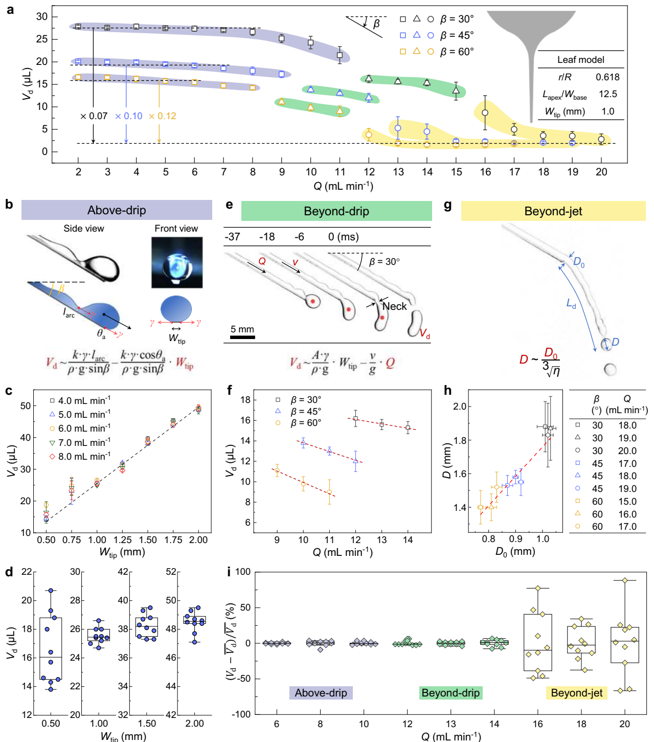
Fig. 3 | Reduced drip volume and stabilized volume deviation of Beyond-drip state. a Variation of drip volume V_d at Q of 2.0–20.0 mL min -1 and \beta of 30–60° of the optimized bodhi leaf apex with r/R = 0.618 , L_{\text{apex}}/W_{\text{base}} = 12.5 and W_{\text{tip}} = 1.0 mm. b Experimental image and scheme of the Above-drip state. c V_d scales with W_{\text{tip}} ( R^2 = 0.98 ) in the Above-drip state ( \beta = 30^\circ ). Dashed line is linear fitting of V_d values with W_{\text{tip}} ranging from 1.0 mm to 2.0 mm. d Box chart of the V_d deviation of different W_{\text{tip}} values. e Drainage dynamics of the Beyond-drip state. Q = 13.0 mL min -1 and \beta = 30^\circ . f V_d scales with Q in the Beyond-drip state. g Image of the Beyond-jet state. The initial water filament diameter D_0 determines the drop
