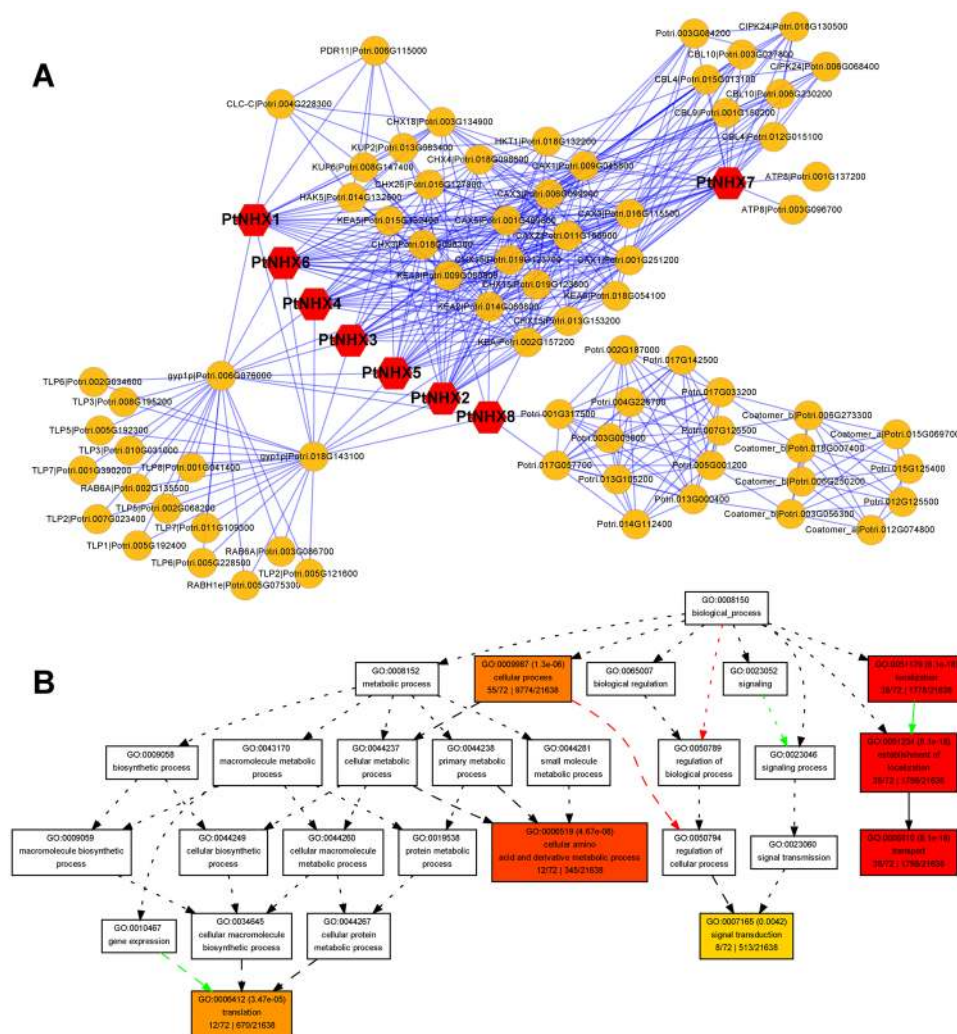
Figure 8. Protein-protein interaction (PPI) network of PtNHXs. (A) PPI network of PtNHX proteins. (B) Enriched BP terms of genes coding the proteins in the PtNHX PPI network. Complement GO enrichment data is shown Fig. S11.
